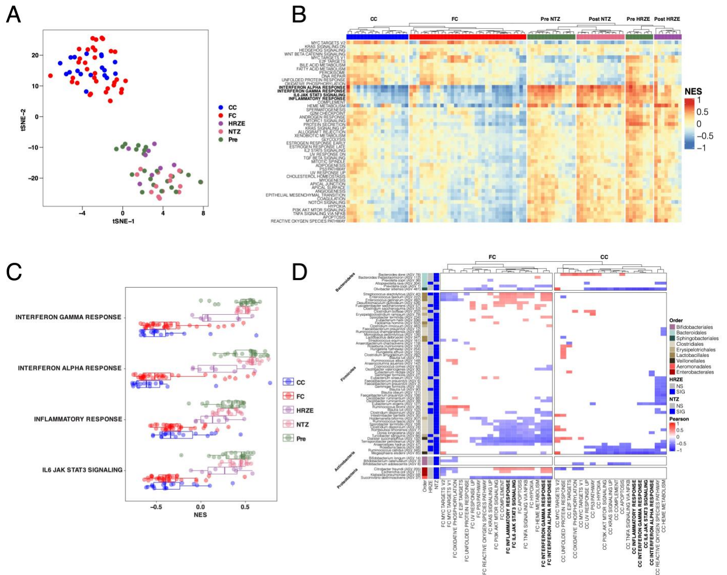
Figure 6: Analysis of microbiome and blood peripheral gene expression in an independent healthy control human cohort validates association between specific microbiome members and host peripheral gene expression. A. t-Distributed Stochastic Neighbor Embedding (t-SNE) ordination all RNAseq samples used in this analysis. This highlights the transcriptional differences between active TB patients, even those on HRZE treatment, and the healthy control cohorts. B. Within-sample GSEA (ssGSEA) of 50 Hallmark pathways from the MiSigDB on a per-sample basis for all cohorts in this study. NES score was calculated using the variance stabilized transformed counts from DSeq, and plotted after scaling across all samples. C. Four representative pathways that correlated with microbiome composition in all cohorts analyzed in this study. D. Pearson's correlations of ASVs with Hallmark pathways in an unbiased fashion highlighting negative correlation of many Clostridia and the proinflammatory pathways highlighted in 6C.
