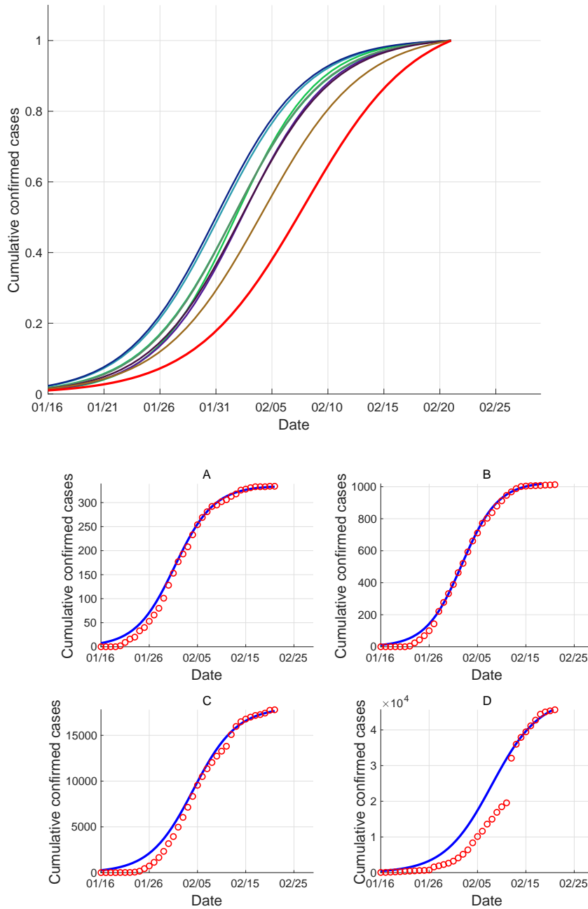
Figure 4: Top:Fitting results of the cumulative number of confirmed cases (normalized) in several areas in mainland China, legend same as in Figure 3; Bottom: Fitting results of the cumulative number of confirmed cases in (A) Shanghai, (B) Hunan, (C) Hubei Province (without Wuhan), (D) Wuhan.
