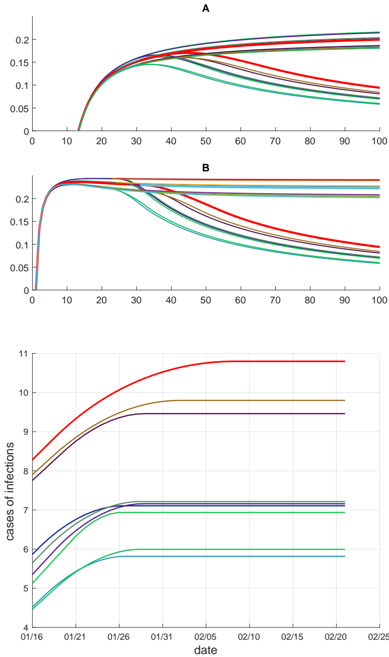
Figure 6: Top: Fitting results of the epidemic evolution in several areas in mainland China, with l_2 = l_1 and l_2 < l_1 . The legend is the same as in Figure 3. (A) The evolution of \frac{1}{t} \ln \left( \frac{J(t)}{J(t_0)} \right) with respect to days started from the first infection date. (B) The evolution of \frac{1}{t} \ln \left( \frac{I(t)}{I(t_0)} \right) with respect to days started from the first infection date. Bottom: Fitting results of log of the
