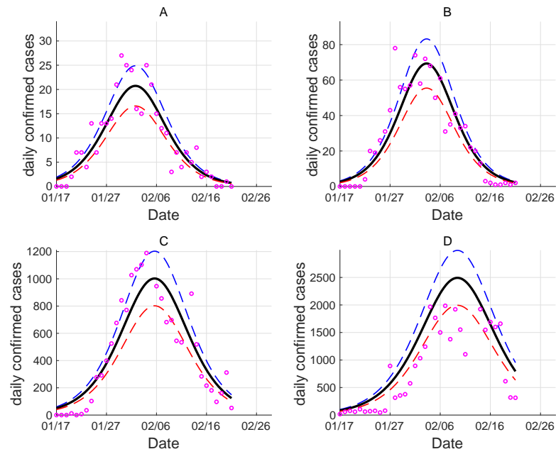
Figure 5: Top:Fitting results of the daily confirmed cases (normalized) in several areas in mainland China, legend same as in Figure 3; Bottom: Fitting results of the daily confirmed cases in (A) Shanghai, (B) Hunan Province, (C) Hubei Province (without Wuhan), (D) Wuhan.
