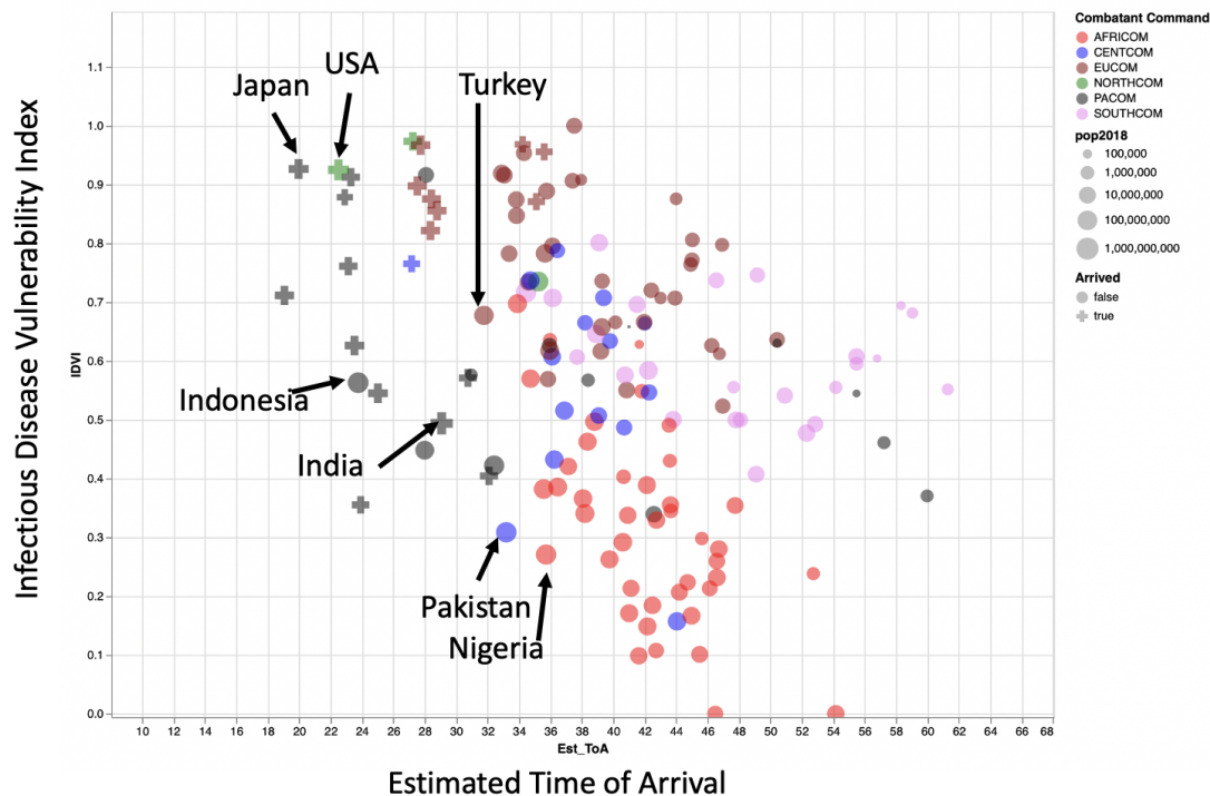
Figure 2. Estimated arrival times based on effective distance to all countries. Countries are colored by the US combatant command. Countries with official confirmed cases as of February 10th are shown with a plus marker. The full interactive visualization is available at https://nssac.github.io/covid-19/import_risk.html
