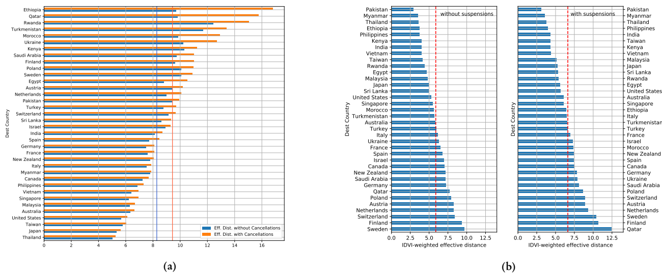
Figure 3. (a) Effective distances to various countries from China with and without airline suspensions (vertical lines indicate the mean effective distance of the displayed countries). (b) IDVI-weighted effective distance index of various countries before and after the airline suspensions.
