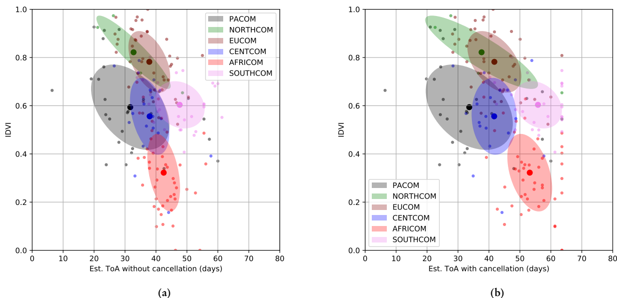
Figure 4. Estimated arrival times vs IDVI (a) without cancellation (b) with cancellation incorporated into the model. The mean-denoted ellipses indicate the standard deviation for the point clouds corresponding to the respective combatant commands.
