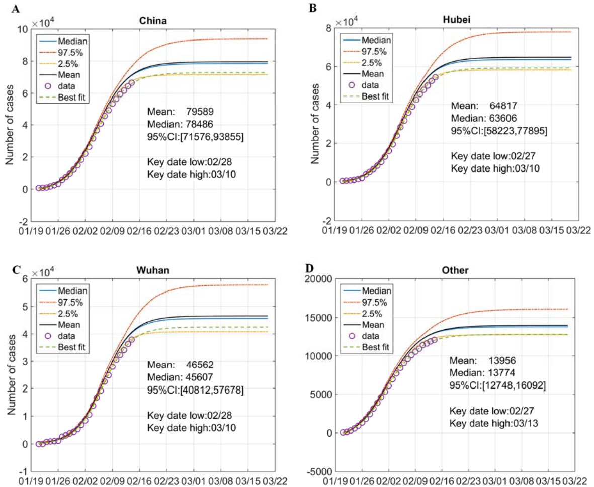
345 346 Figure 3. Analysis of the uncertainty of confirmed cases for mainland China, Hubei 347 Province, Wuhan City and other provinces.
