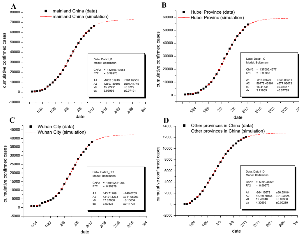
327 Figure 1. Fitting the cumulative number of confirmed cases from mainland China to 328 Boltzmann function
