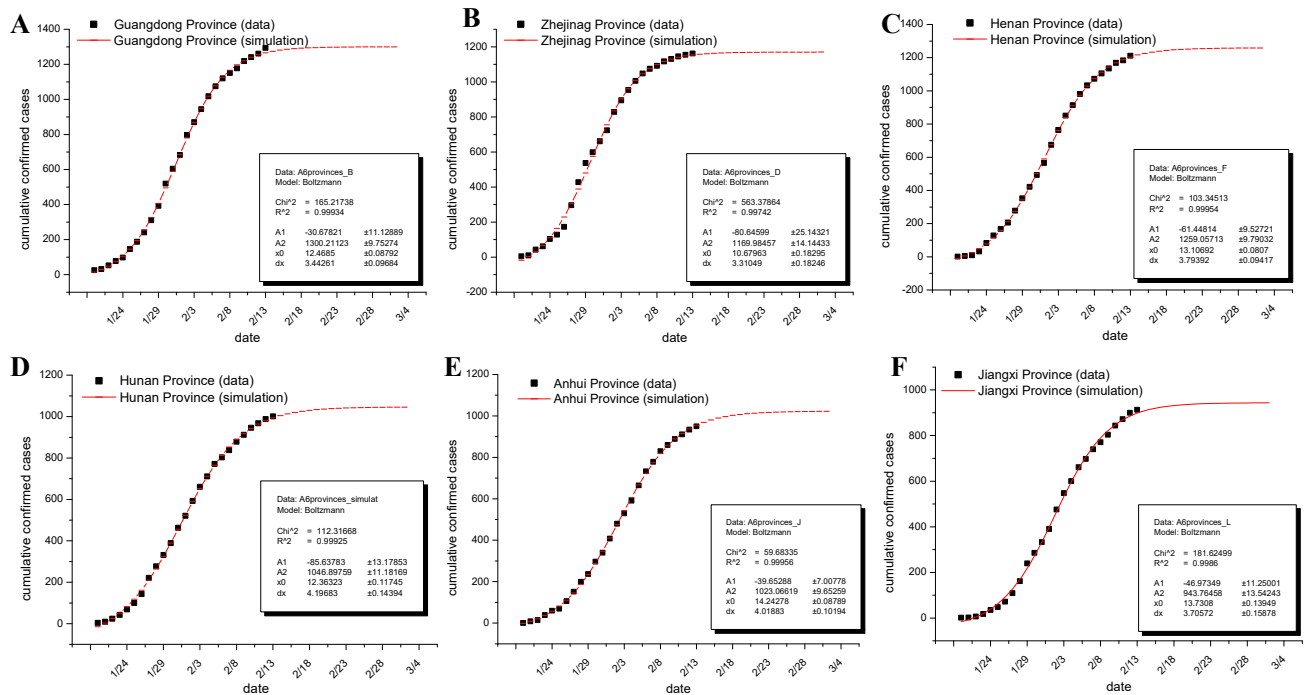
338 Figure 2. Fitting the cumulative number of confirmed cases from the six most affected 339 provinces to Boltzmann function
