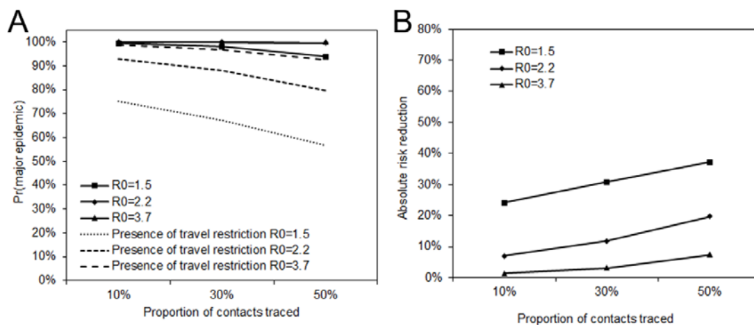
Figure 3. Probability of a major epidemic with various levels of transmissibility and traced contact.
