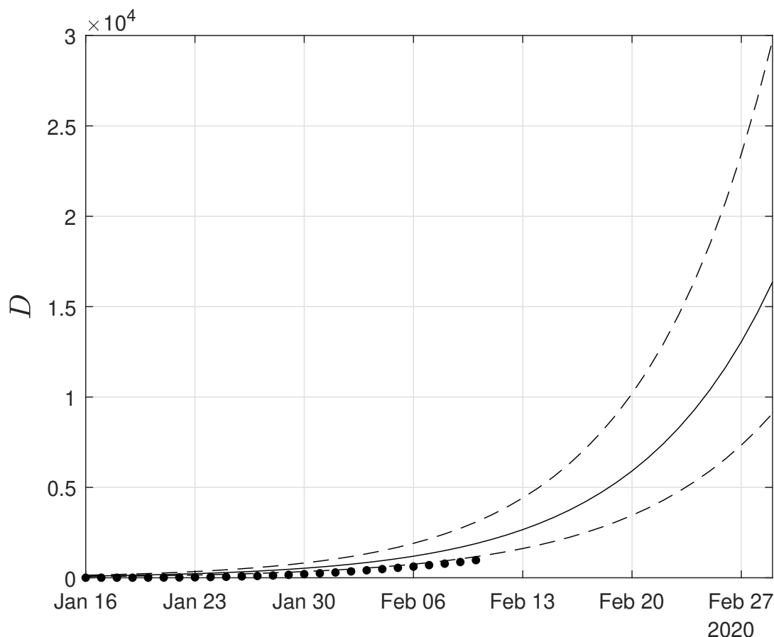
Figure 8: Scenario I. Simulations until the 29th of February of the cumulative number of deaths as obtained using the SIRD model. Dots correspond to the number of confirmed cases from 16th of January to the 10th of February. The initial date of the simulations was the 16th of November with one infected, zero recovered and zero deaths. Solid lines correspond to the dynamics obtained using the estimated expected values of the epidemiological parameters \alpha = 0.199 , \beta = 0.05 , \gamma = 0.0294
