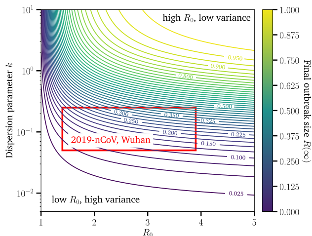
FIG. 2. Final size of outbreaks with different R_0 and distributions of secondary cases. We use a negative binomial distribution of secondary cases and scan realistic range of parameters. Most importantly, the range of parameters corresponding to the current outbreak of 2019-nCoV is highlighted by a red box. The range of potential R_0 comes from a 95% confidence interval using an early data and a classic deterministic models [18, 19]. The range of dispersion parameter k comes from analogy with severe acute respiratory syndrome [13, 24]. Most importantly, with fixed average, the dispersion parameter is inversely proportional to the variance of the underlying distribution of second cases.
