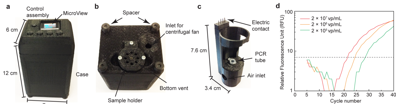
Figure 1. 3D manufactured real-time PCR device for rRT-PCR-based virus detection. (a) The amplification and fluorescence reading status is displayed in real time. (b) The bottom view showing an air inlet for the centrifugal fan. (c) The sample holder holds the PCR tube. (d) rRT-PCR Fluorescence readings show the shift in the intensity measurements corresponding to the differing concentrations of virus. Reprint from [22].
