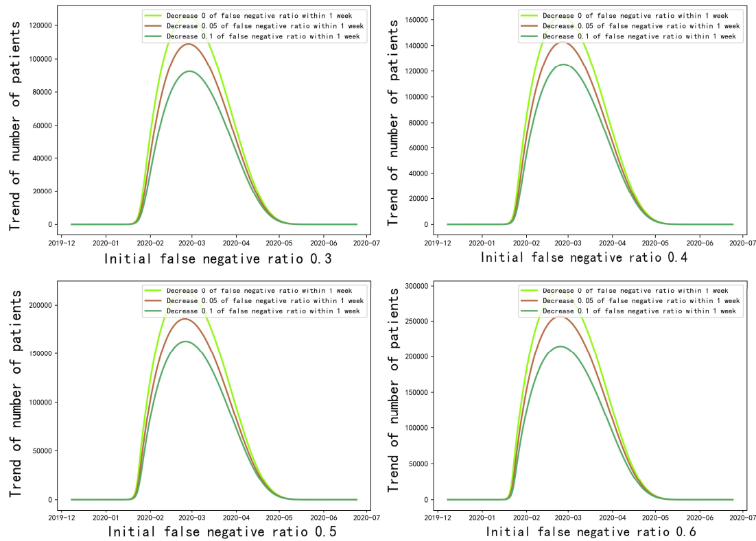
Figure 10. Estimation of the real number of patients with different decrease on false negative ratio (0%, 5%, 10%) within a week.
