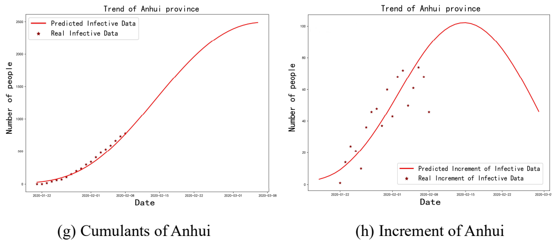
Figure 6. Comparisons between the predicted infective data and the real infective data
