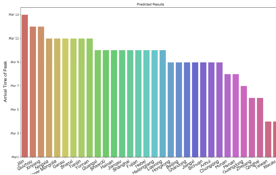
Figure 3. Predicted arrival time of peak number of confirmed cases in each province of China, the x-axis corresponds to different geographical areas and the y-axis is the prediction of peak arrival time at average level.
