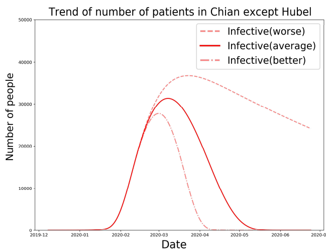
Figure 8. Iteration results of the number of confirmed cases in China except Hubei.
