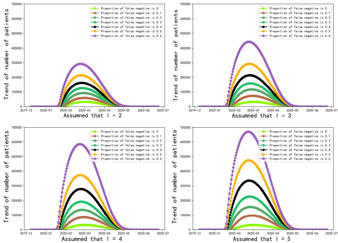
Figure 9. Estimation of the real number of patients with different l (2, 3, 4, 5)
