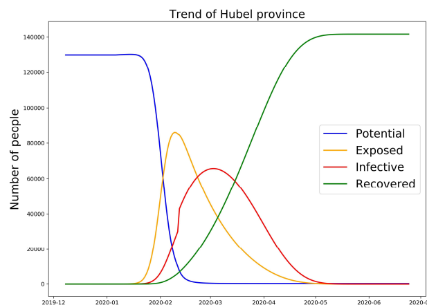
Figure 4. Simulated epidemic trend of Hubei with \tau = 0.9 and \varepsilon = 0.25
