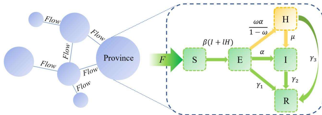
Figure 1. Flow-SEHIR Model Diagram
