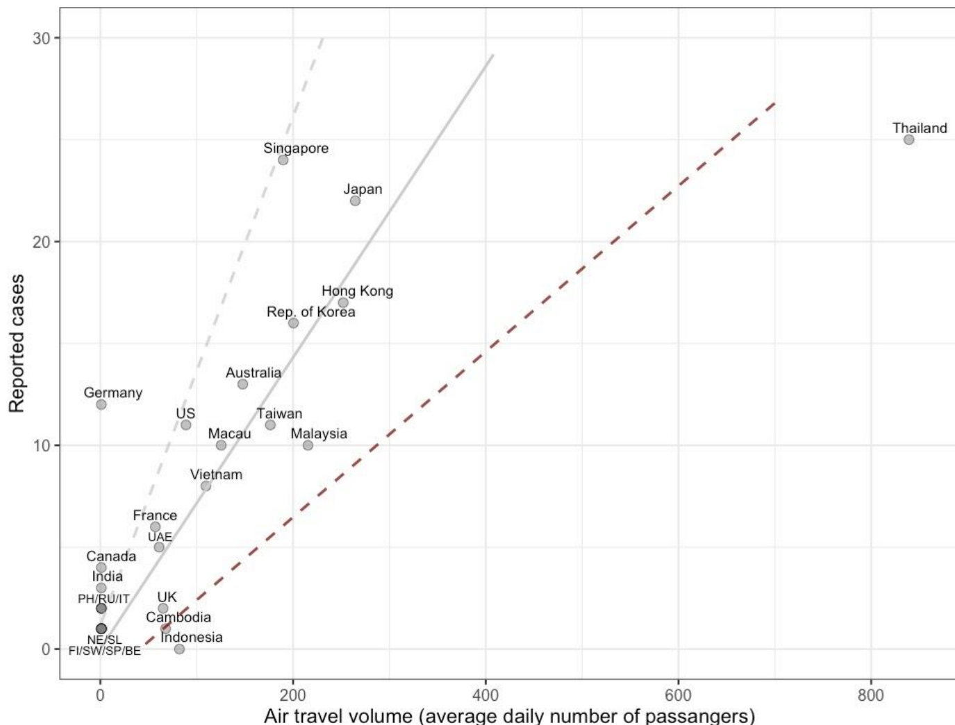
Figure 1 Reported case counts and air travel volume. The solid line shows the expected case counts based on our model, and the dashed lines show the 95% prediction interval bounds (grey dashed line for the upper bound, red for the lower bound). The Philippines (PH), Russia (RU) and Italy (IT) all report two cases each. Nepal (NE), Sri Lanka (SL), Finland (FI), Sweden (SW), Spain (SP) and Belgium (BE) all report one case each. Other abbreviations: United Arab Emirates (UAE), United States of America (US).
