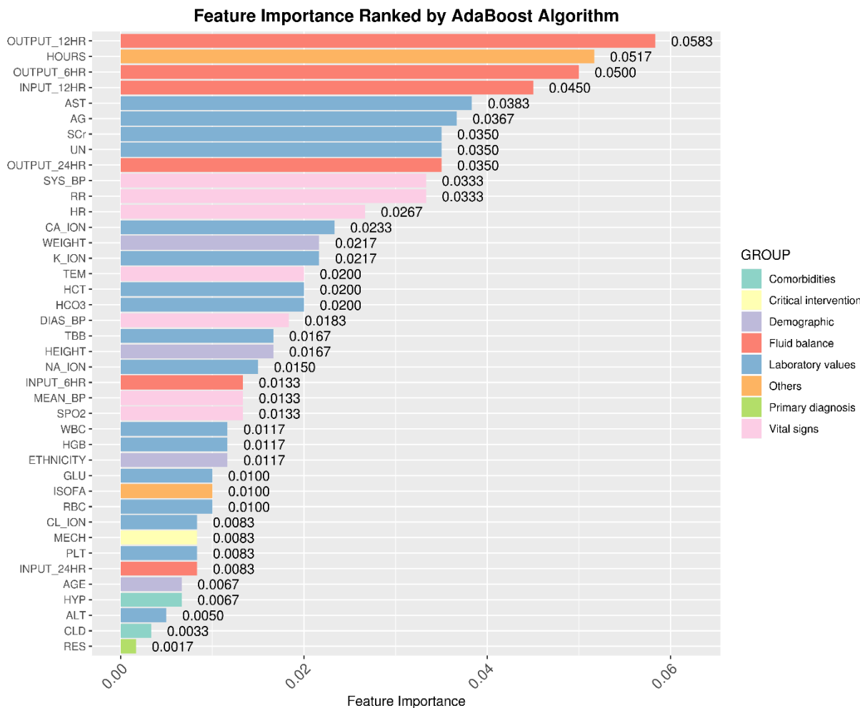
400 401 Figure 6. Identified top important features in eICU database. Values and rankings are based on 402 time-series model 6-6 and the averaged Gini importance from AdaBoost algorithm. Features are 403 colored group-wisely according to the categories listed in Table 1. The higher value indicates the 404 higher significance of the feature.
