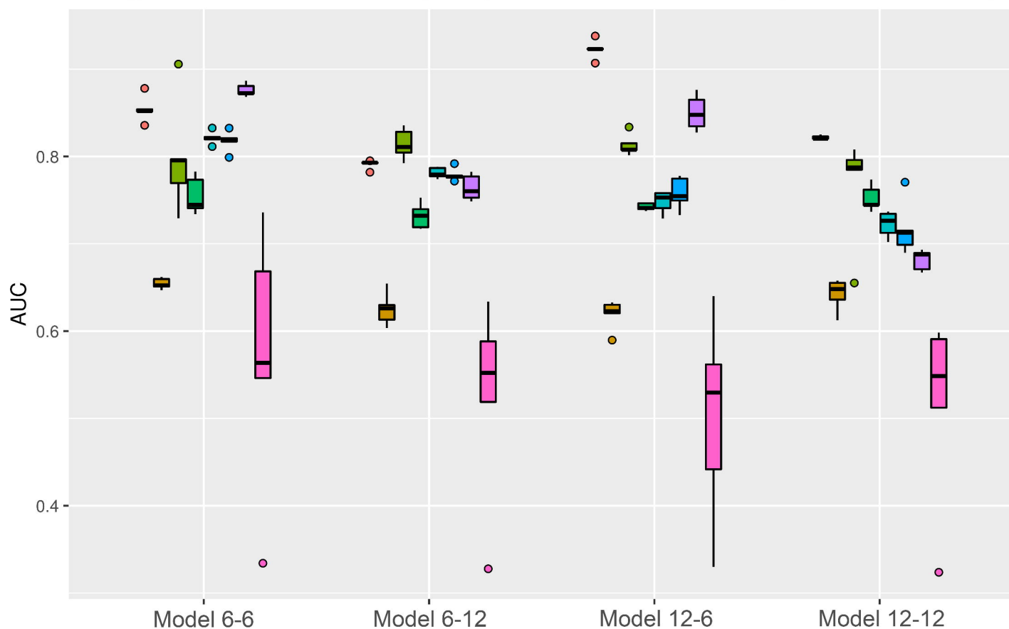
B Algorithm Performances (AUC) with Different Models (MIMIC Database)
