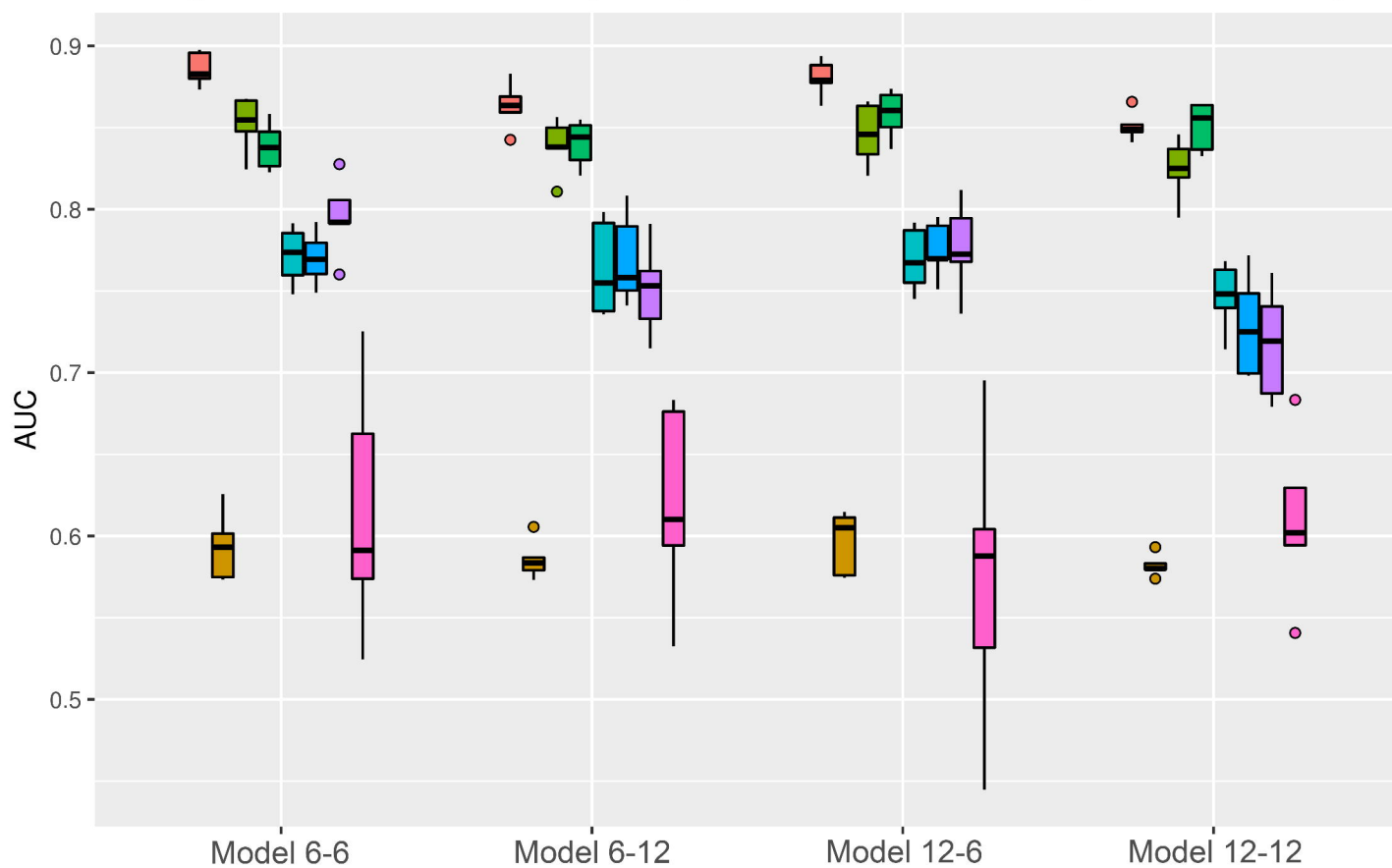
A Algorithm Performances (AUC) with Different Models (EICU Test Set)
