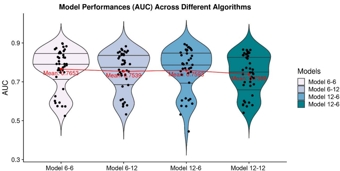
376 377 Figure 5. Model performances (AUC) violin plot of four different configurations of the models 378 (model 6-6, model 6-12, model 12-6, model 12-12) across eight different algorithms with five- 379 fold cross-validation. Black solid horizontal lines in each violin plot are the interquartile range 380 lines. Red points and lines indicate the mean performances (AUC) over four models.
