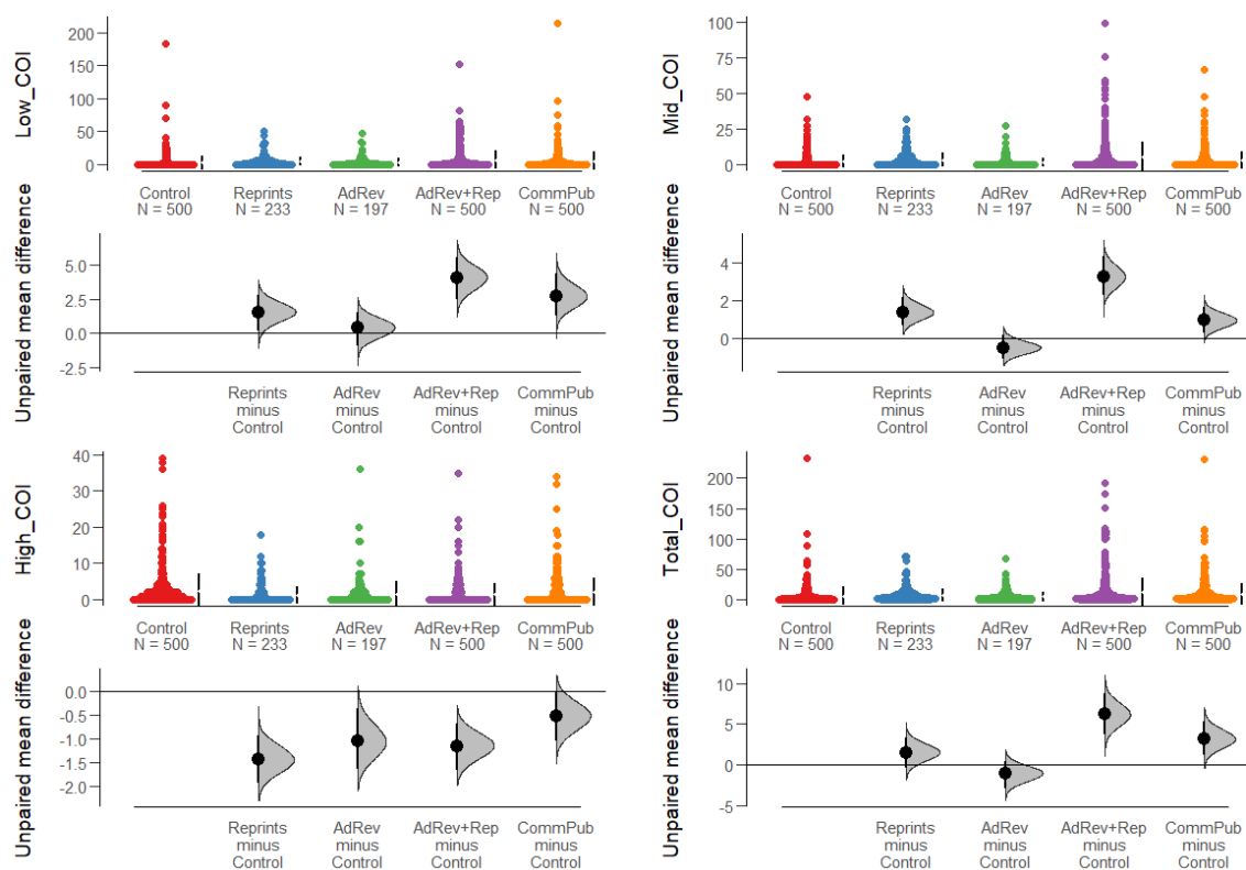
Figure 1: Shared-Control Estimation Plots for aCOI by level and total aCOI.
