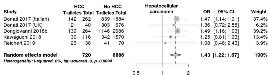
Figure 5. rs641738C>T is associated with higher odds of NAFLD-HCC.
