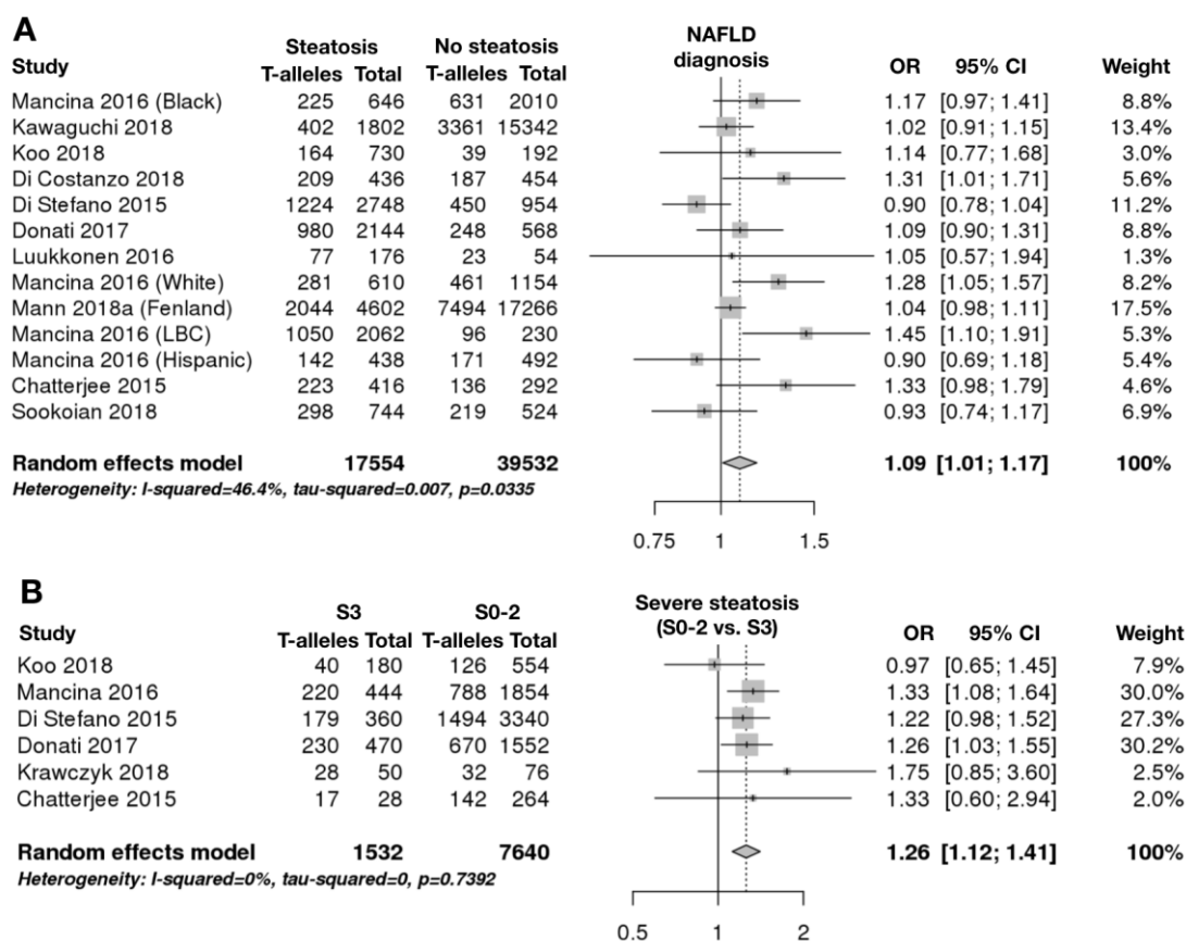
Figure 2. rs641738C>T is associated with higher odds of diagnosis of NAFLD and histological severity of steatosis. Data from 28,543 adults with radiologically defined steatosis for presence versus absence of NAFLD (2A), and from 4,572 adults with liver biopsy data for presence of severe steatosis (S0-2 versus S3, 2B) using an additive model of inheritance.
