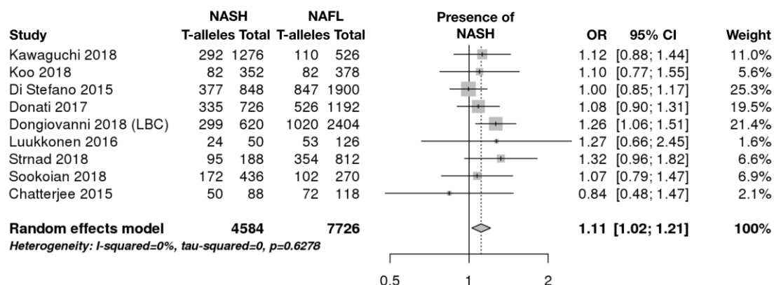
Figure 3. rs641738C>T is associated with higher odds of NASH on biopsy. Data from 6,155 adults with NASH defined according to the FLIP algorithm for NAFL versus NASH, using an additive model of inheritance. NAFL, non-alcoholic fatty liver.
