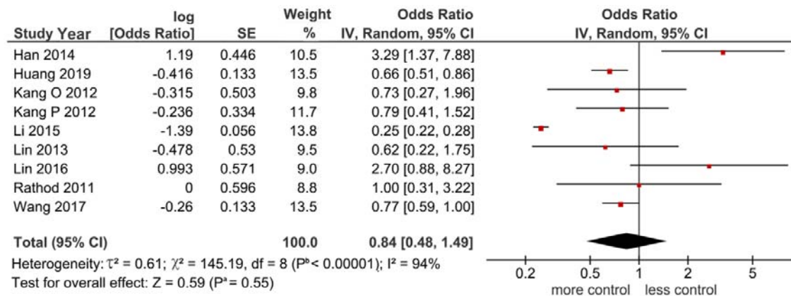
322 Fig 4 Forest plot outcome in the CEE analysis
