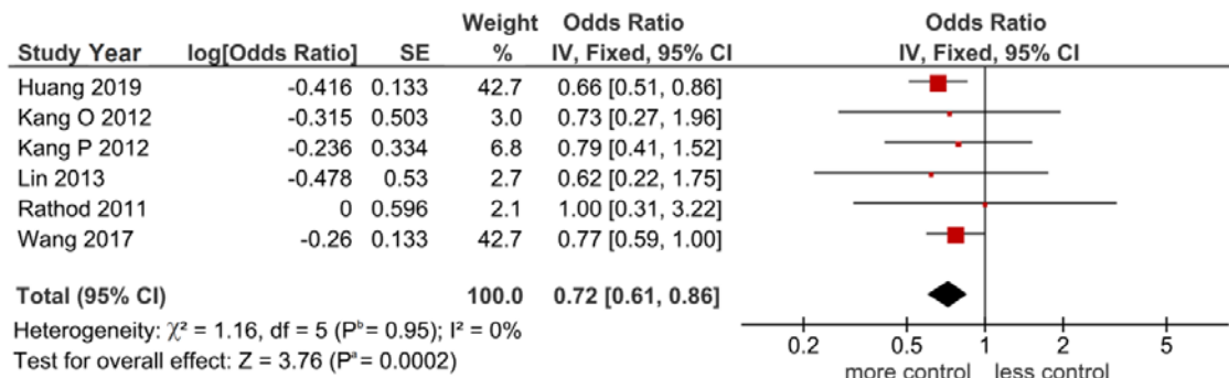
344 Fig 6 Forest plot outcome of outlier treatment in the CEE analysis
