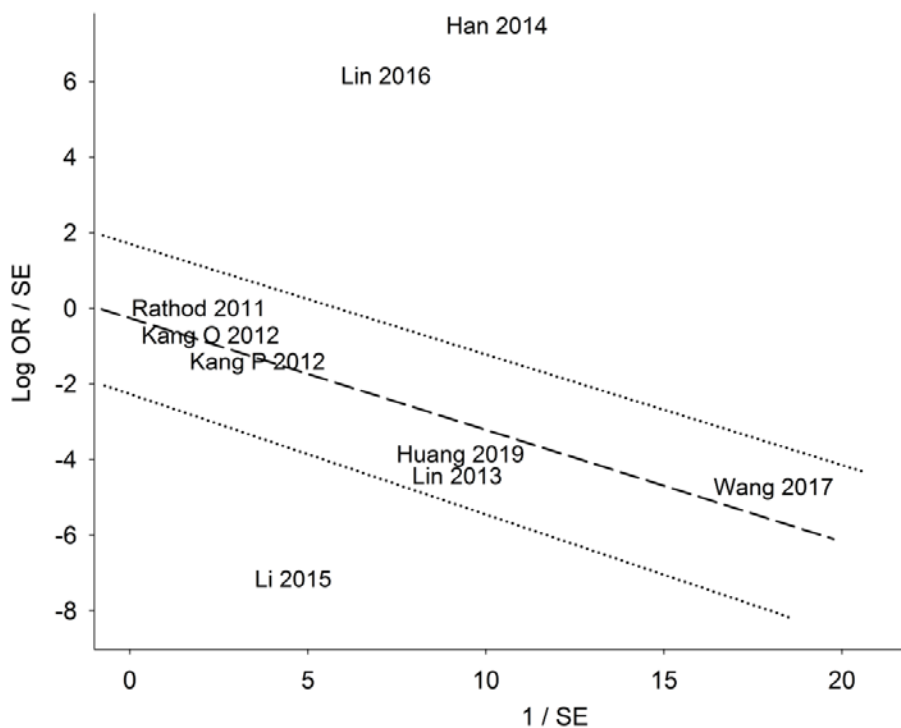
337 Fig 5 Galbraith plot in the CEE analysis
