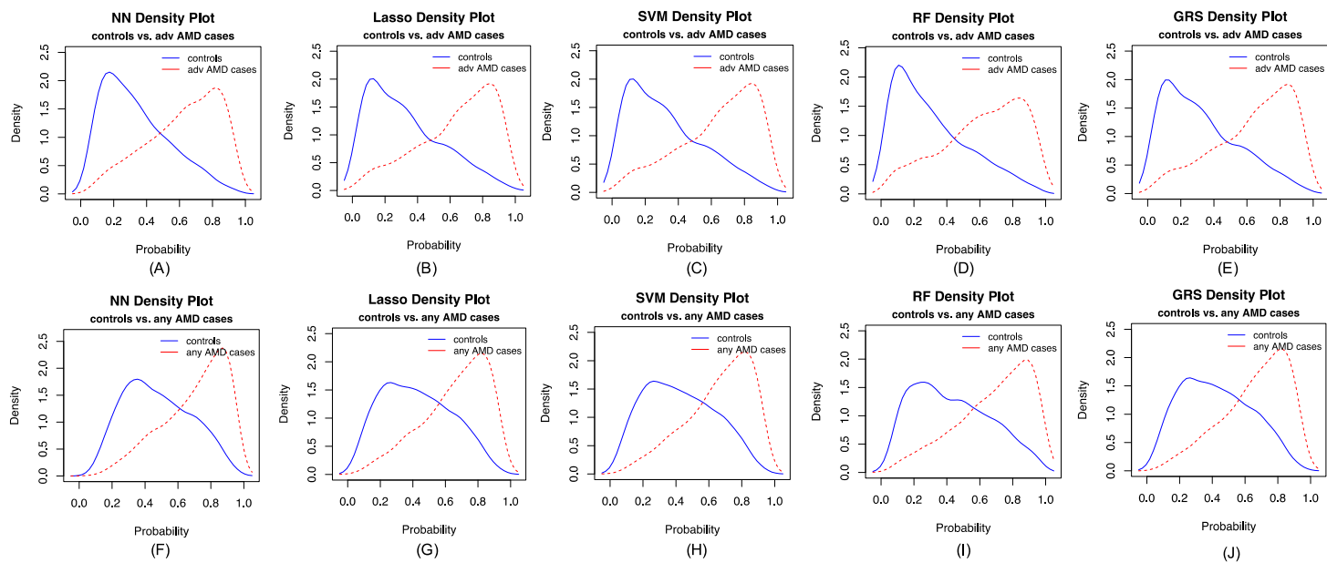
Figure 3. Density curves of the predicted risk for the two counterparts for five prediction methods. (A-E) normal controls vs. advanced AMD cases, and (F-J) normal controls vs. any AMD cases.
