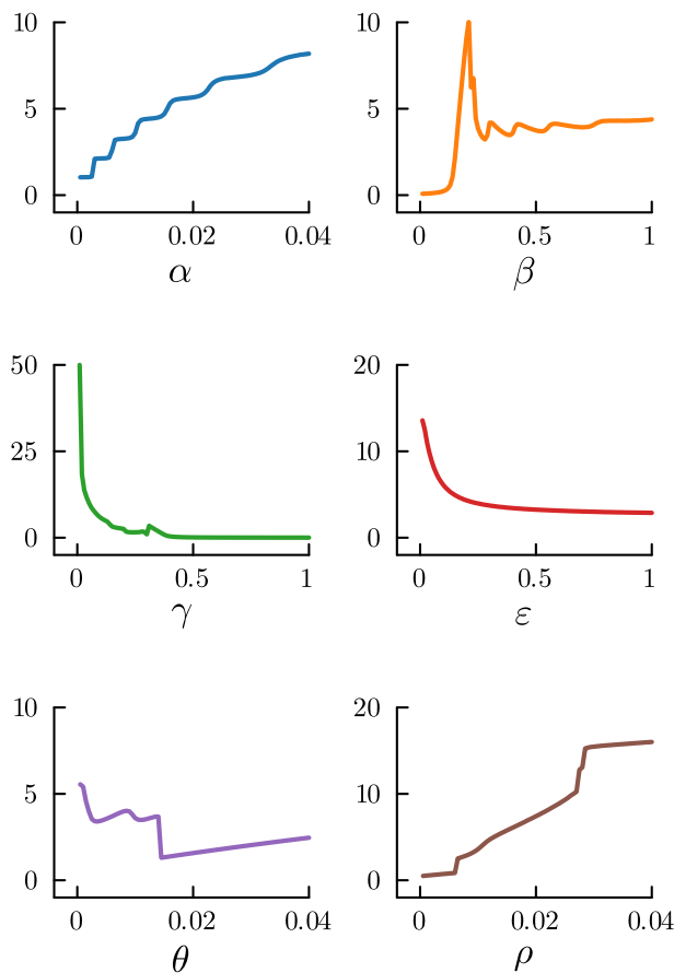
Figure 2: Infection load ( y axes) for varying parameters \alpha, \beta, \gamma, \epsilon, \theta , and \rho . When varying a parameter, the others are fixed and taken from Table 1.
