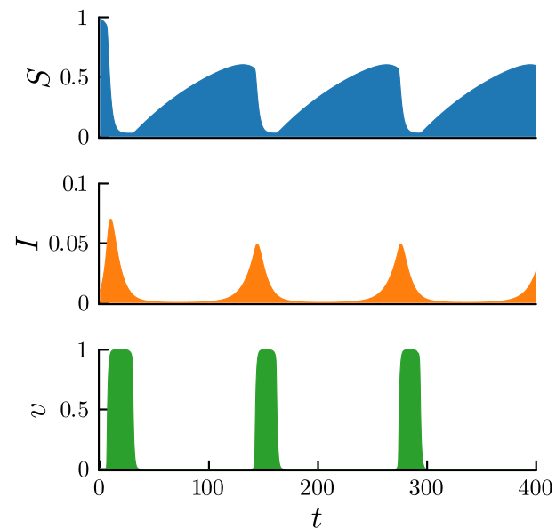
Figure 1: A representative example of observed cycles. Rising infections sway susceptibles to become vaccinated, which drives down infections. In turn, the vaccination rate declines. As immunity wanes, susceptibles rise and the process repeats. Initial conditions are S_0 = 0.99 , I_0 = 0.01 , and v_0 = 0.01 and parameter values are taken from Table 1.
