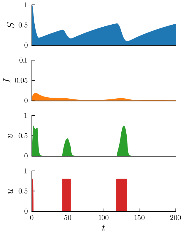
Figure 3: Numerically solved optimal control solution. Initial conditions are S_0 = 0.99 , I_0 = 0.01 , and v_0 = 0.01 . w = 0.01 and u_{\max} = 0.8 . Other parameter values are taken from Table 1.
