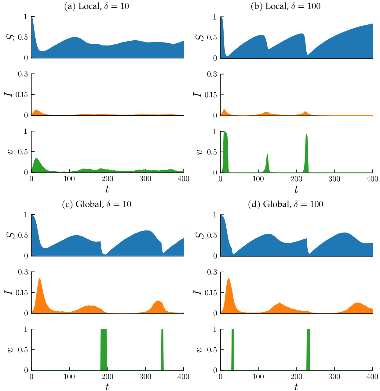
Figure 4: Representative time series for the network model with local or global knowledge of disease prevalence and vaccine uptake levels. Initial conditions are S_0 = 0.99 , I_0 = 0.01 , and v_0 = 0.01 . Parameter values are from Table 1.
