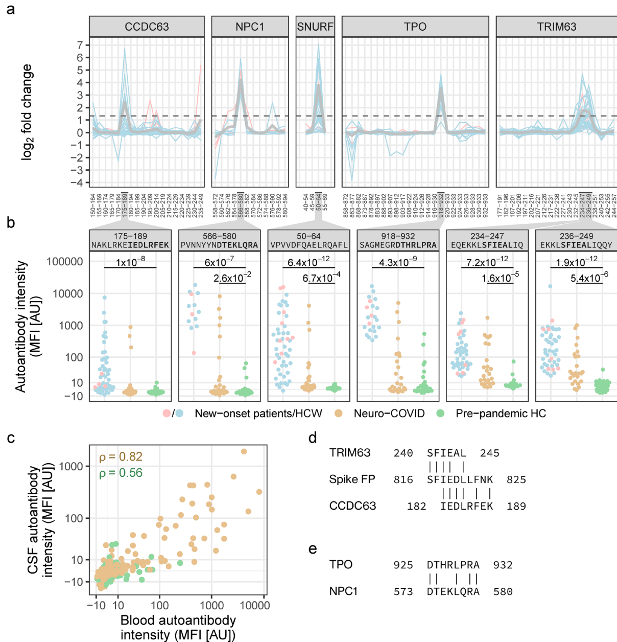
Fig. 4 | The main epitopes of new-onset autoantibodies are elevated in blood and CSF of an independent cohort with neuro-COVID and display molecular mimicry with the SARS-CoV-2 fusion peptide. a Epitope mapping revealed the main epitopes of six new-onset autoantibodies. Lines depict epitope profiles (anti-peptide IgG log 2 FC) at new-onset in individuals with the corresponding new-onset autoantibody. Gray lines depict the mean. The dashed line indicates the cutoff for classification as a main epitope (FC ≥ 2.52). Numbering on the x-axis corresponds to the peptide amino acid positions in the full-length protein (Table S3). b Antibodies against the main epitopes were elevated in an independent cohort of neuro-COVID patients compared to pre-pandemic HCs. Brackets indicate statistically significant difference to pre-pandemic HC (q-values \leq 0.05 from Mann-Whitney U-test with Benjamini-Hochberg correction). The y-axis displays signal intensity on the pseudo-log 10 scale. c Correlation of autoantibodies in blood and CSF of neuro-COVID patients and pre-pandemic HCs. Data points correspond to paired blood and CSF samples in neuro-COVID patients (n=23) and HCs (n=21), and the peptides shown in panel b. \rho : Spearman's rho. d,e Sequence similarity between d the main epitopes of TRIM63 and CCDC63 to the SARS-CoV-2 fusion peptide, and e between the main epitopes of TPO and NPC1.
