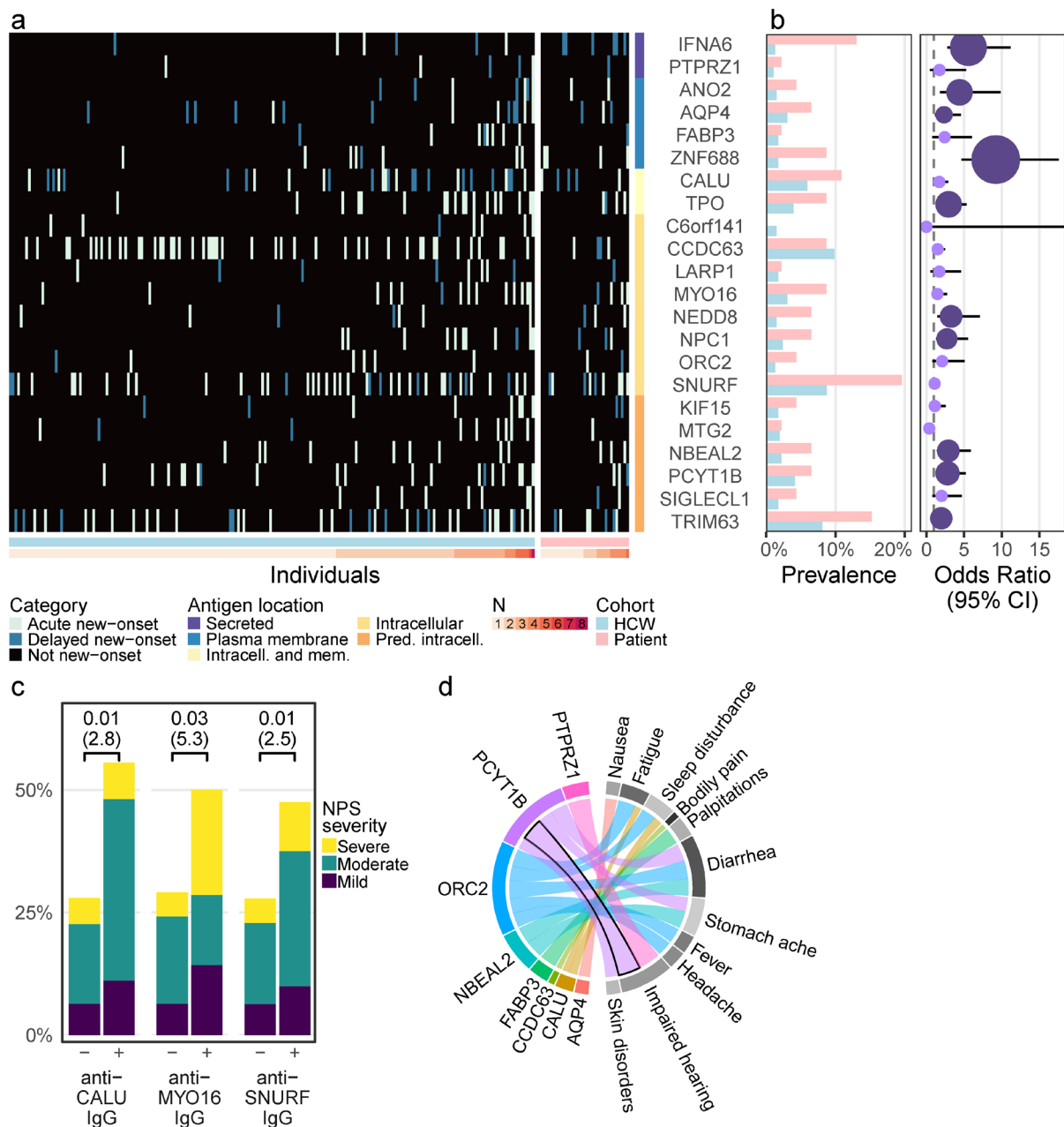
Fig. 2 | New-onset autoantibodies have increased prevalence in hospitalized COVID-19 patients and are associated with neuropsychiatric symptoms post-COVID-19. a Overview of new-onset autoantibodies in HCW and hospitalized COVID-19 patients. The 22 prevalent new-onset autoantibodies are grouped by their antigen location. Columns show individuals with at least one prevalent new-onset autoantibody. Cell color represents new-onset autoantibody category: Acute, delayed, or not new-onset. b Hospitalized COVID-19 patients showed increased prevalence of nearly half of the most prevalent new-onset autoantibodies. Bars indicate autoantibody prevalence in patients (pink) and HCW (blue). Point position and lines indicate odds ratio with 95% confidence interval (CI) based on logistic regression. Point size and color shows magnitude of q-value (Benjamini-Hochberg). Light purple: q > 0.05 . Dark purple: q \leq 0.05 . c Increased severity of neuropsychiatric symptoms post-COVID-19 was associated with three new-onset autoantibodies. Bars depict proportions of HCW with different severities of neuropsychiatric symptoms post-COVID-19 among autoantibody-positive (+) and negative (-) groups. Brackets indicate p-values and odds ratios (in parentheses) from proportional odds logistic regression. d Eleven symptoms post-COVID-19 were associated with eight of the most prevalent new-onset autoantibodies. Band widths indicate the estimated logit (log odds ratio) of associations with p \leq 0.05 . The indicated association of PCYT1B and impaired hearing remained significant after Benjamini-Hochberg correction ( q = 0.002 ).
