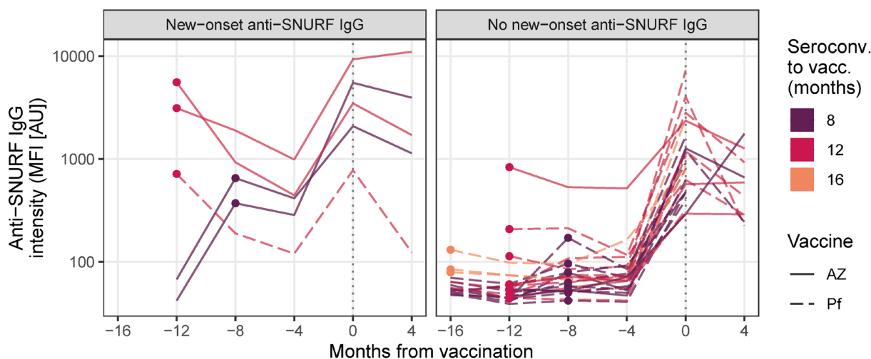
Fig. 3 | Increasing levels of anti-SNURF IgG at vaccination. Line plots depicting individuals with a 4-fold increase of anti-SNURF IgG at vaccination vs 4 months prior. The x-axis shows time centered on time of first vaccination (dashed vertical line). Individuals are separated across panels based on whether they developed new-onset anti-SNURF IgG at seroconversion (i.e. prior to vaccination). Line color indicates time between seroconversion and first vaccination, and points display time of seroconversion.
