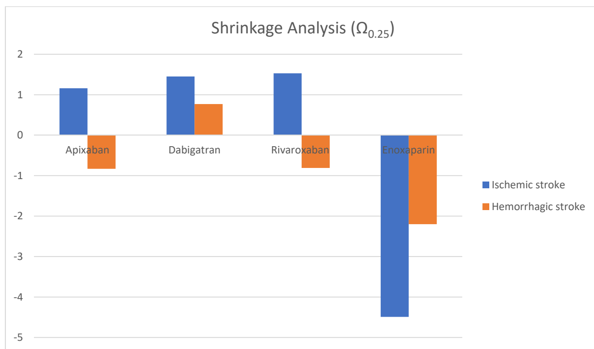
Figure 1: Shrinkage Analysis for the Anticoagulants-Levetiracetam Interaction
