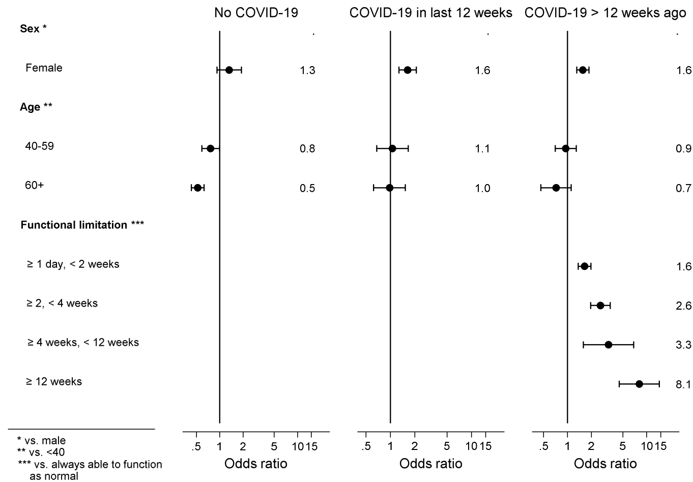
Fig. 3. Associations with symptom pattern 2 (vs. symptom pattern 1) meta-analysed across studies. Bars represent 95% confidence intervals. Estimates are from random effects meta-analyses of study-specific estimates.
