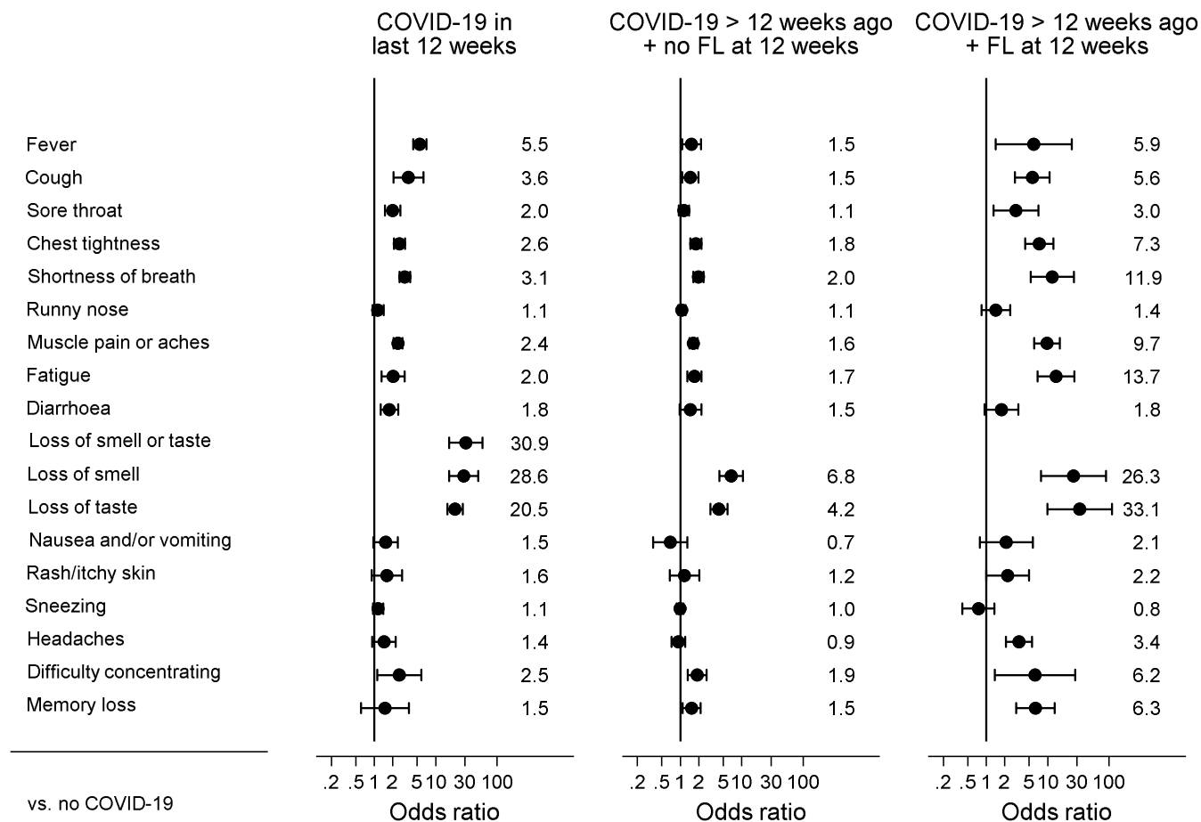
Fig. 1. Odds ratio of each symptom for each COVID-19 group relative to the no COVID-19 group. Bars represent 95% confidence intervals. Estimates are from random effects meta-analyses of study-specific estimates.
