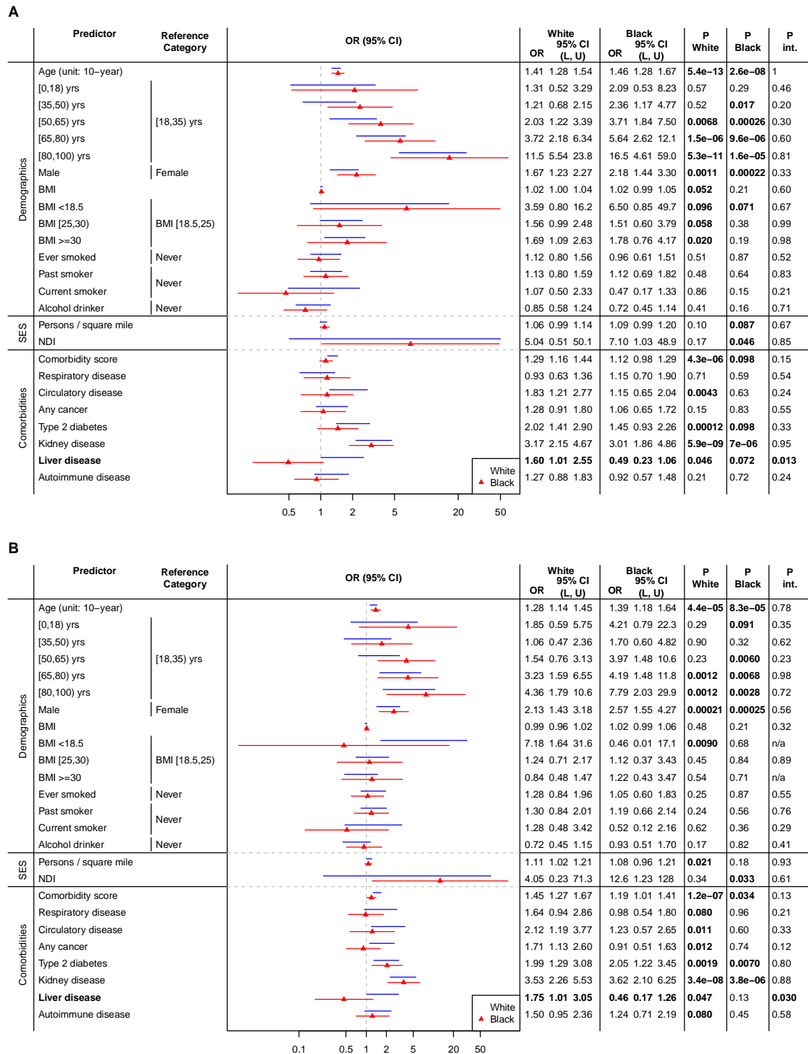
Figure 2. Hospitalization (A) and ICU Admission (B) for Black and White Patients in the Full Cohort. Abbreviations: BMI, body mass index; NDI, Neighborhood Socioeconomic Disadvantage Index. The results were from model \text{logit } P(Y_{COVID} = 1|X, \text{Covariate}) = \beta_0 + \beta_X X + \beta_{Race} \text{Race} + \beta_{int} X \times \text{Race} + \beta_{Cov} \text{Covariate} , where Y_{COVID} denotes hospitalization (A) or ICU admission (B), and \text{Covariate} = \text{age} + \text{sex} + \text{NDI} (+ comorbidity score in the demographic and socioeconomic status models). Results that are statistically significant at the level of 0.05 are bolded.
