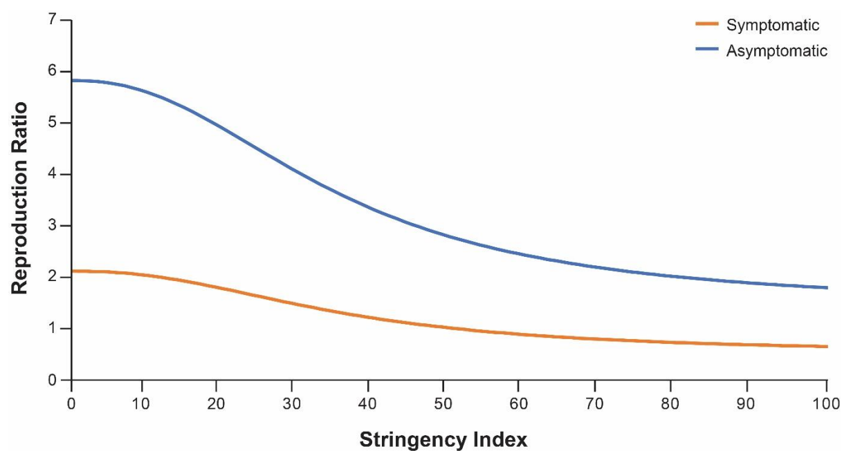
Figure 3. Relationship between the stringency index and the reproduction ratio.
