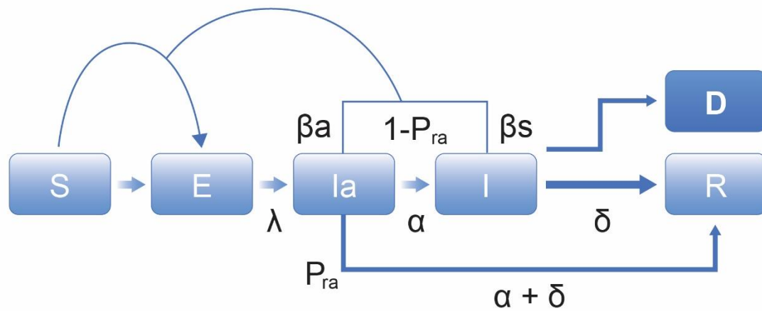
Figure 1. Initial COVID-19 transmission model.
