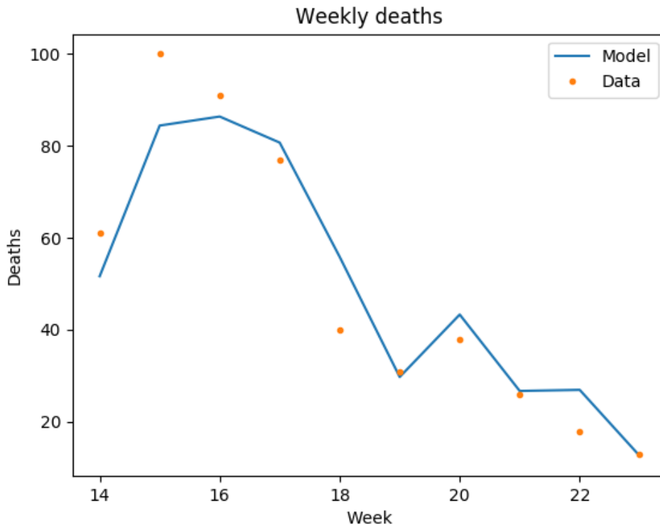
Figure 8: Model and data for the weekly deaths. Weeks are counted starting on the week ending on April 3rd, 2020.
