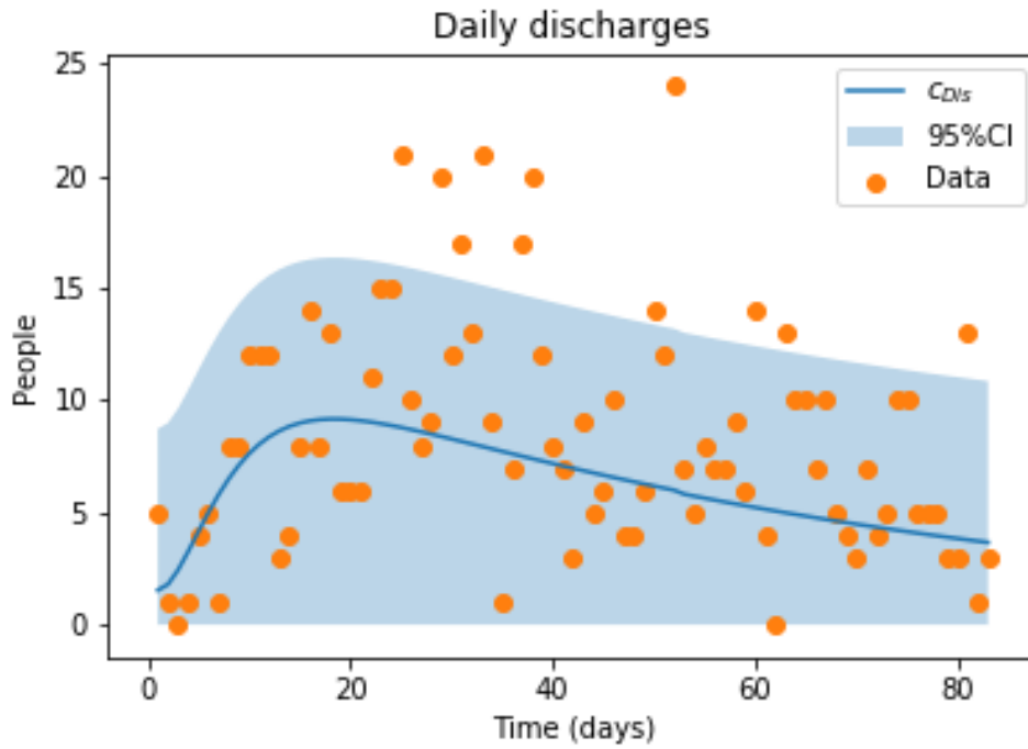
Figure 3: Results of fitting the reduced model defined by (.37) for discharges. The blue line depicts c_{Dis} , the light blue region depicts the 95% confidence interval and the orange points represent the data set C_{Dis} .
