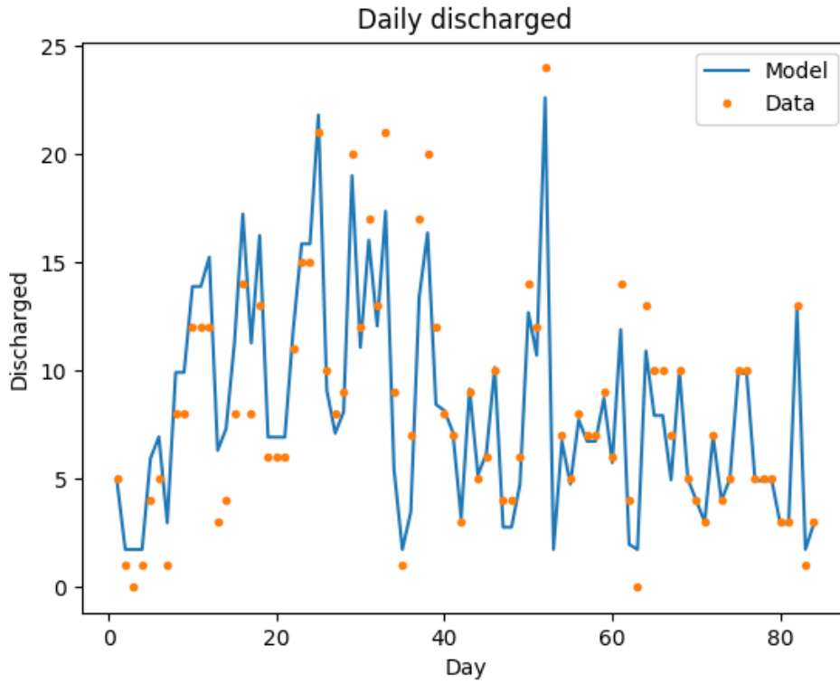
Figure 7: Model and data for the daily discharged patients. Days are counted starting on March 24th, 2020.
