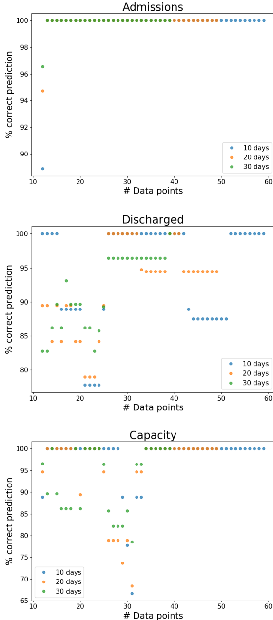
Figure 5: Predictive power of the SEIR-D model for East Sussex, West Sussex and Brighton and Hove, evaluated as the percentage of days predicted within a 95% accuracy.
