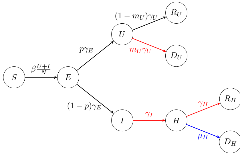
Figure 1: Schematic diagram illustrating the transmission dynamics within the population in the South East region of the UK (Brighton and Hove, East and West Sussex). All arrows indicate the flow of data from one compartment to the other. Colour code: Black arrows indicate the flow with no reliable datasets, red and blue arrows indicate the flow with reliable datasets (hospital and non-hospital). All parameters in the diagram are assumed unknown and must be obtained as part of the model solution procedure (see Sections 3 for details).
