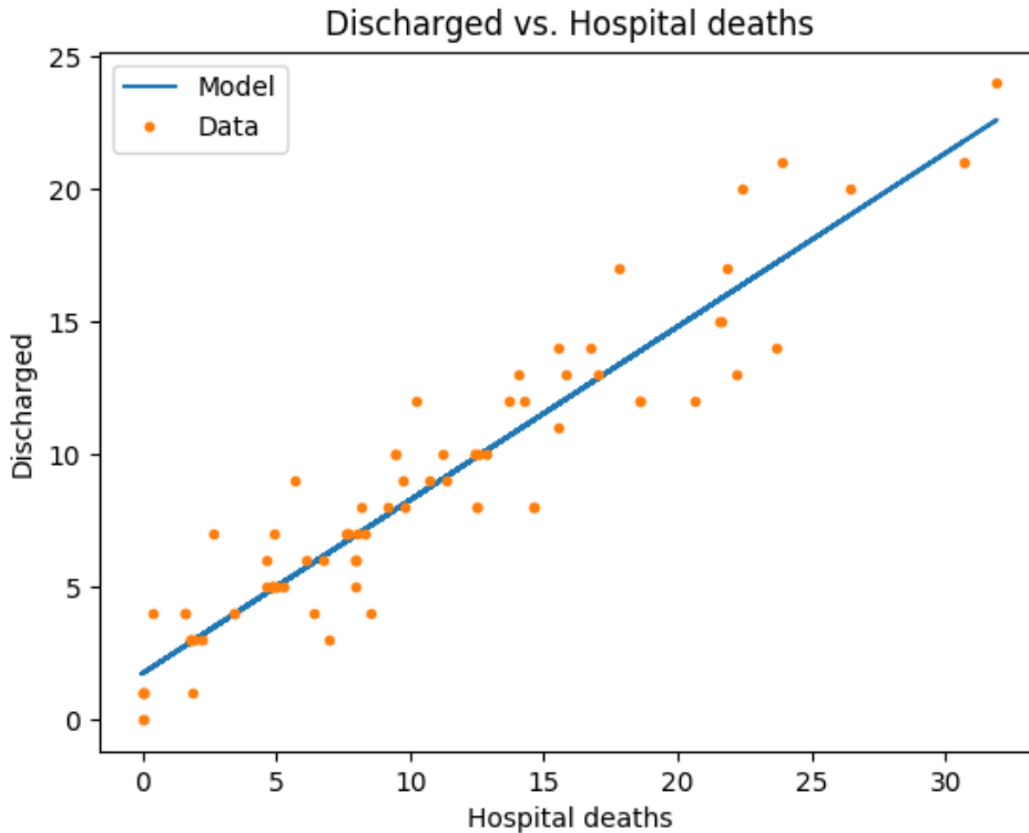
Figure 6: Model and data for the daily discharged patients and daily deaths. Note that only discharged data is available daily; the corresponding daily deaths were inferred (see Figure 8).
