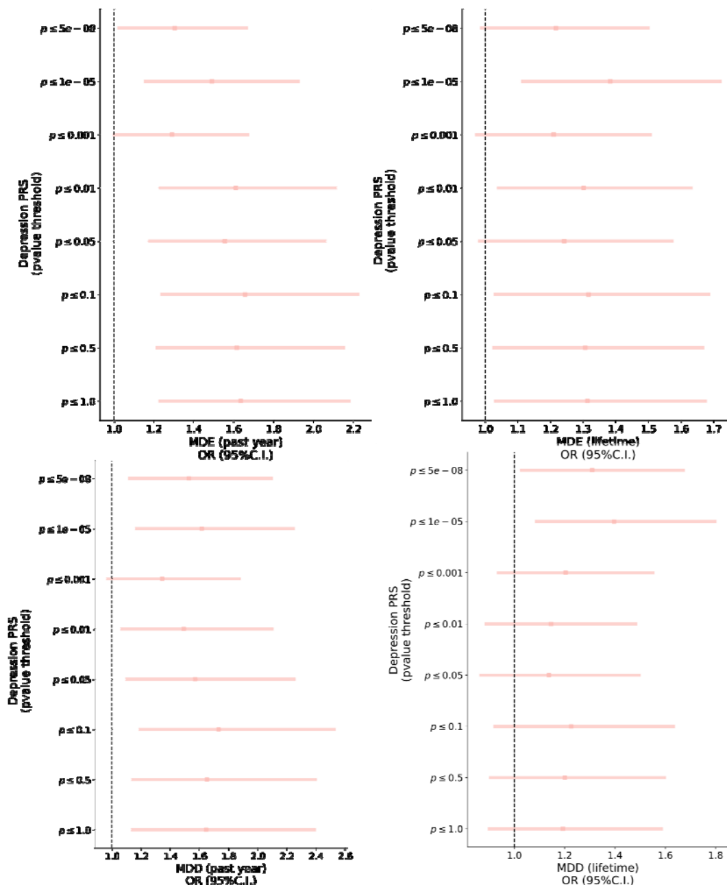
Fig. 1. Depression PRS and phenotypic depression associations
