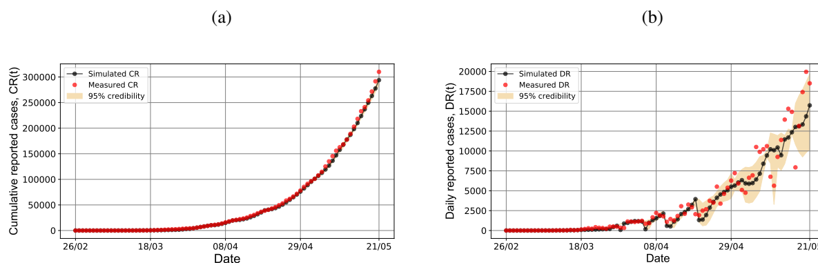
Figure 7: Monitoring results for (a) cumulative cases and (b) daily reported cases from the PF simulations, considering data from February 26, 2020 up to May 21, 2020 in Brazil.
