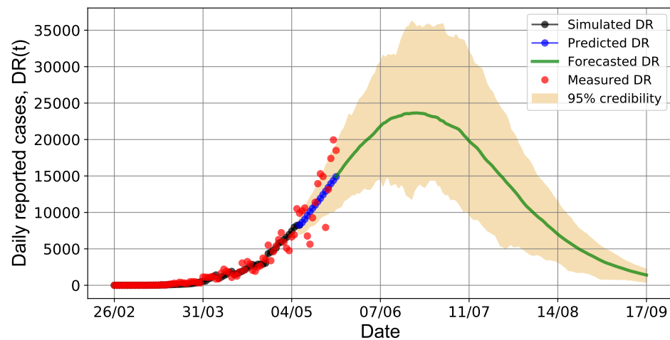
Figure 12: Forecast result for the daily reported cases in Brazil up to September 17, 2020.
