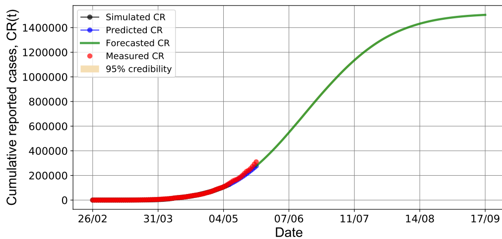
Figure 14: Forecast result for the cumulative reported cases up to September 17, 2020.
