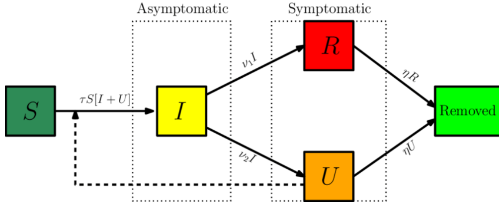
Figure 2: Flow chart illustrating the infection path process.
