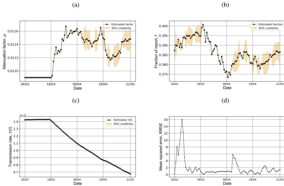
Figure 8: Dynamic results of the SIRU model parameters: (a) attenuation factor, \mu ; (b) fraction of report, f(t) = f_0 ; (c) transmission rate, \tau(t) = \tau_0 \exp[-\mu(t - N)] ; and (d) the mean squared error, RMSE, from the PF simulations, considering data from February 26, 2020 up to May 21, 2020 in Brazil.
