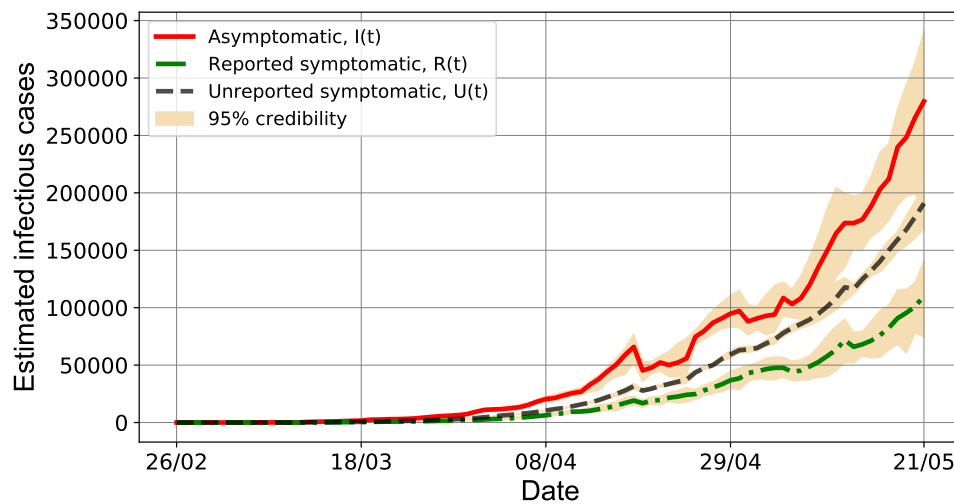
Figure 9: Monitoring results for reported and unreported cases from the PF simulations, considering data from February 26, 2020 up to May 21, 2020 in Brazil, for asymptomatic and symptomatic infectious cases, I(t) , R(t) and U(t) .
