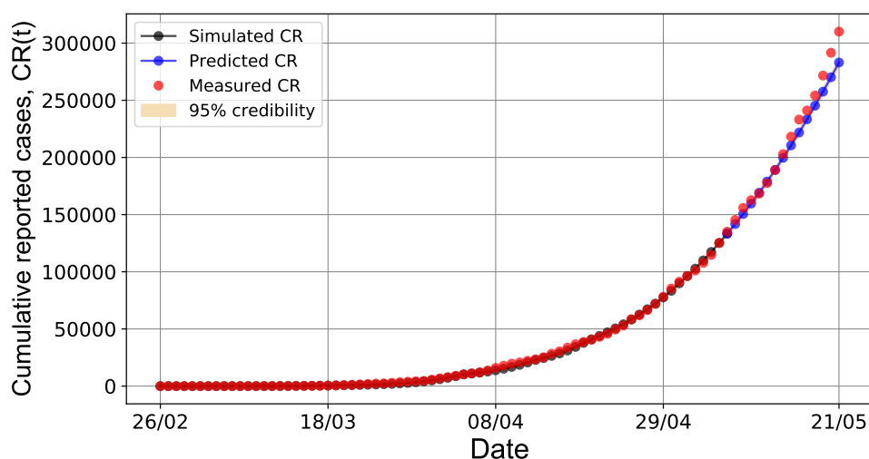
Figure 10: Validation of the predictive capability of the PF simulations for the measured number of reported cases in Brazil, considering data from May 08, 2020 up to May 21, 2020.
