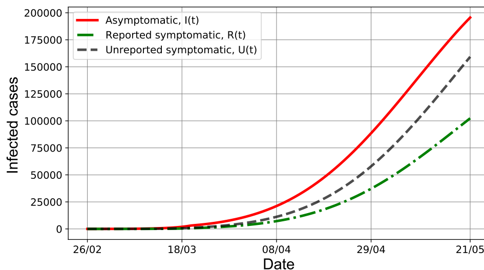
Figure 5: Monitoring results for reported and unreported cases from PSO simulations, considering data from February 26, 2020 up to May 21, 2020 in Brazil, for asymptomatic and symptomatic infectious cases, I(t) , R(t) and U(t) , with f_0 = 0.39123 , \mu = 0.0109 and \tau_0 = 1.426 \cdot 10^{-9} .
