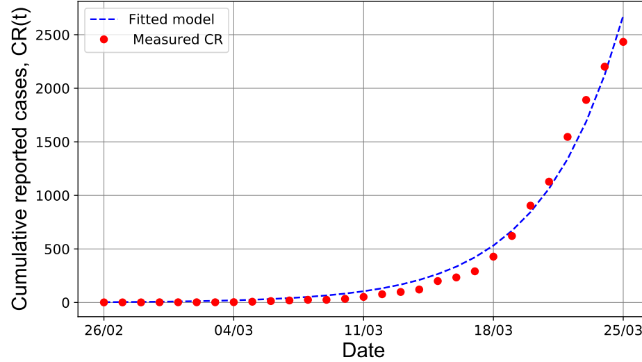
Figure 3: Early stage fitting for the cumulative reported cases, CR(t) = \chi_1 \exp(\chi_2 t) - \chi_3 , in Brazil from February, 26 2020 up to March 25, 2020, with \chi_1 = 4.185 , \chi_2 = 0.231 , and \chi_3 = 1.0 .
