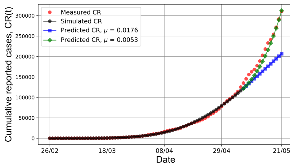
Figure 6: Simulation and prediction results from PSO simulations compared with the measured number of reported cases in Brazil from May 08, 2020 up to May 21, 2020. Different changes on were carried out to improve the performance of the prediction step.
