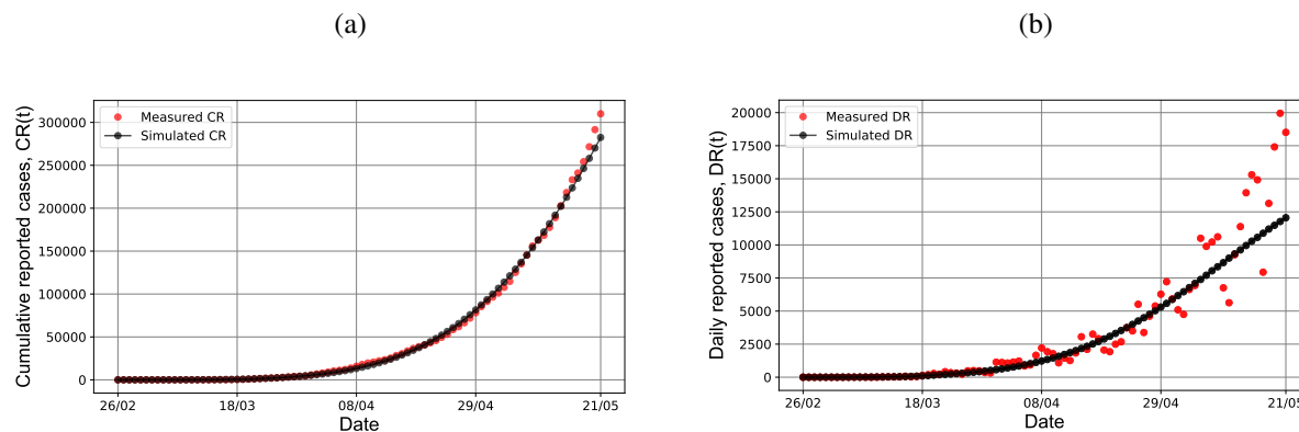
Figure 4: Monitoring results for cumulative (a) and daily (b) reported cases from PSO simulations, considering data from February, 26 2020 up to May 21, 2020 in Brazil, with f_0 = 0.39123 , \mu = 0.0109 and \tau_0 = 1.426 \cdot 10^{-9} .
