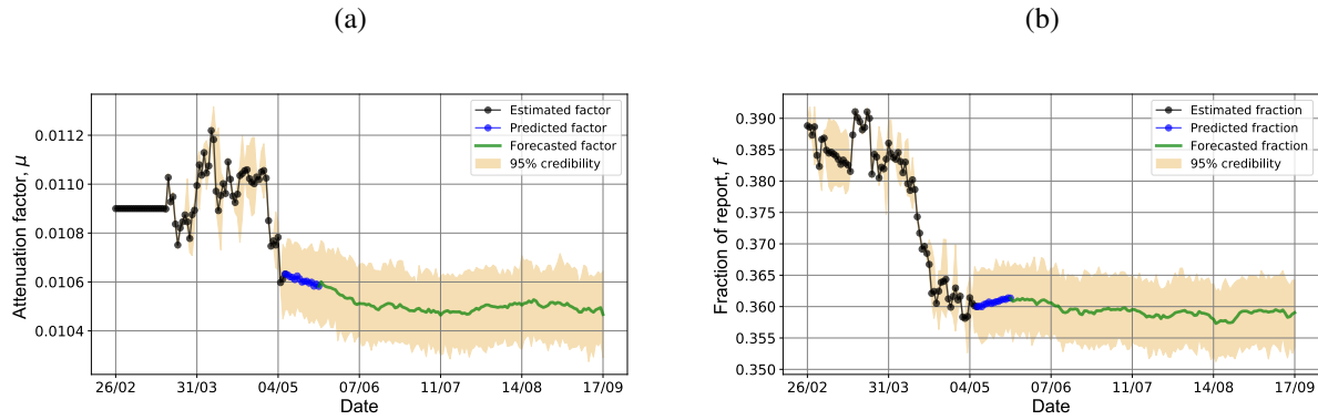
Figure 11: Dynamic behaviour of the parameters during the prediction and forecasting steps: (a) attenuation factor, \mu ; (b) fraction of report, f(t) = f_0 .
