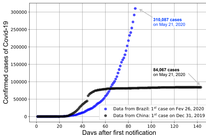
Figure 1: Comparison between the number of confirmed cases of Covid-19 in Brazil (85 days since first case) and in China (142 days since first case) up to May 21, 2020.
