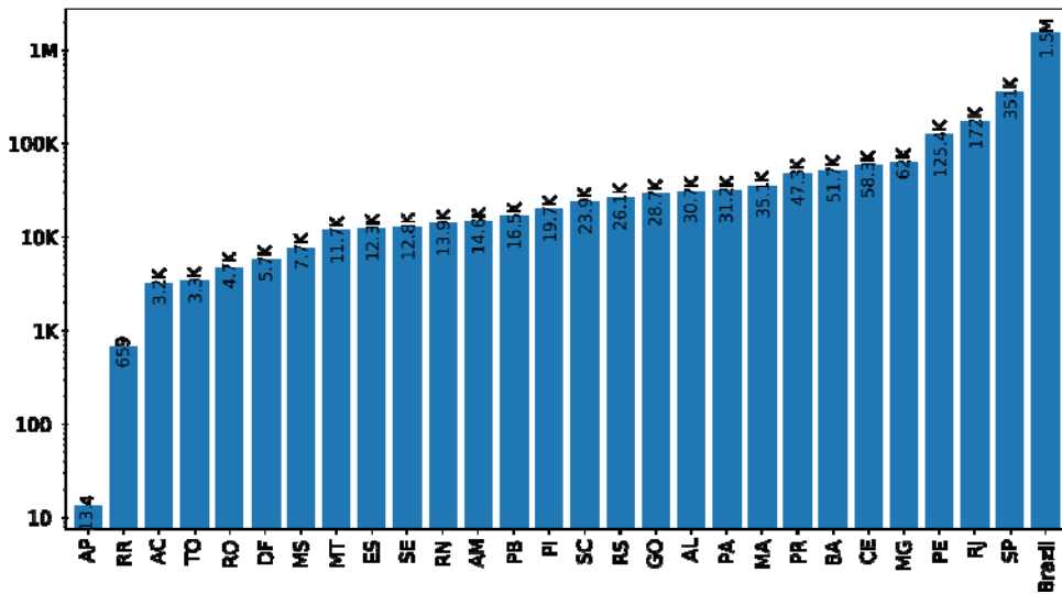
Fig 25 Total estimated deaths based on SUQC mode
