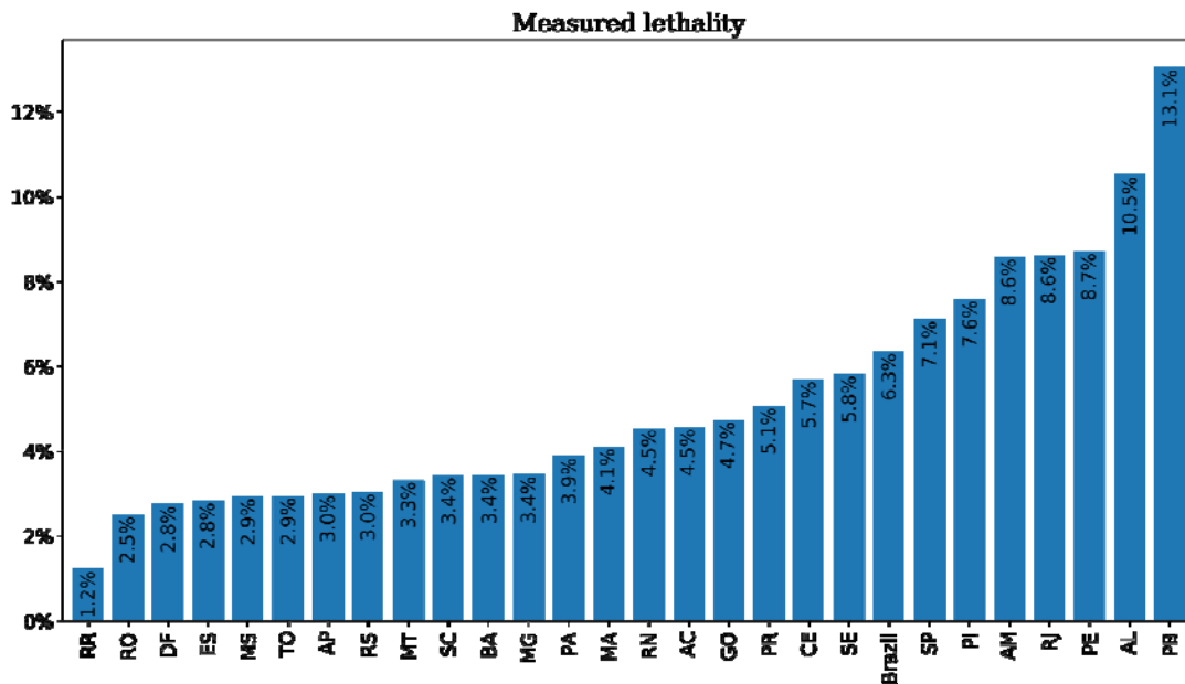
Fig 30 Total deaths per total confirmed cases
