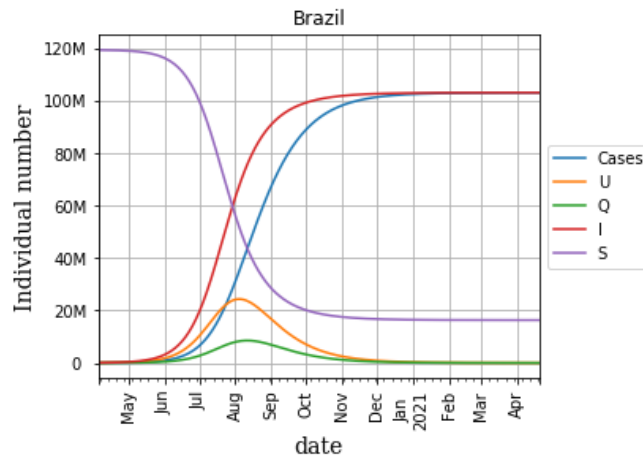
Fig 26 SUQC model of Brazil
