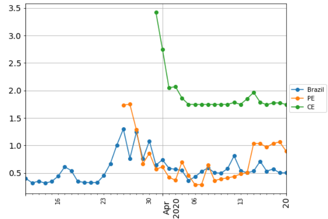
Fig 21 Growth rate (interval of 15 days) based on GRM model
