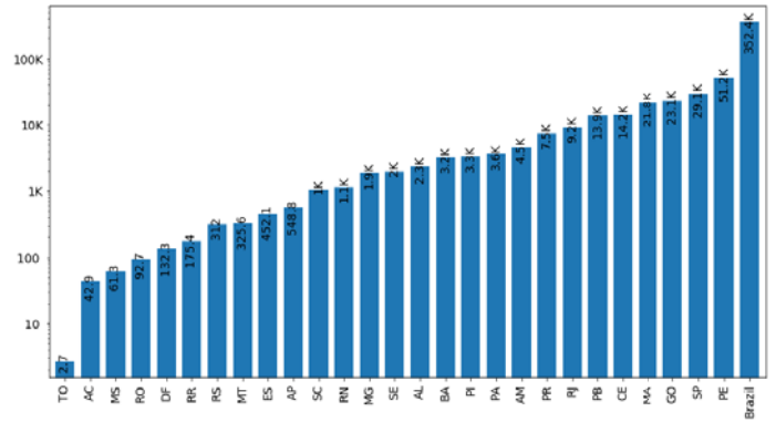
Fig 24 Total estimated deaths based on GRM model
