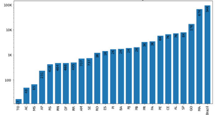
Fig 18 Maximum number of daily cases based on GRM model
