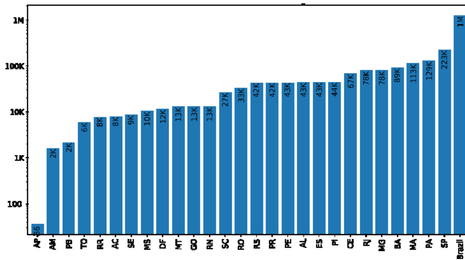
Fig 19 Maximum number of daily cases based on SUQC model
