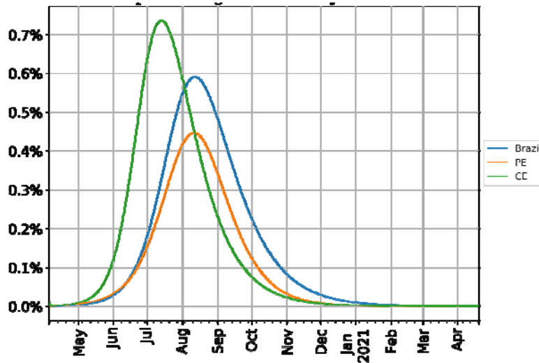
Fig 13 Percentage of daily cases based on SUQC model
