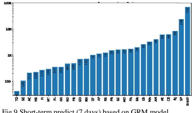
Fig 9 Short-term predict (7 days) based on GRM model
