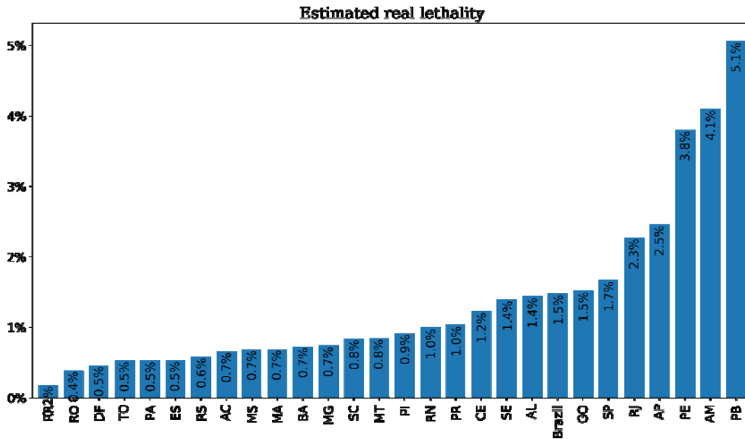
Fig 31 Total deaths per all infected cases
