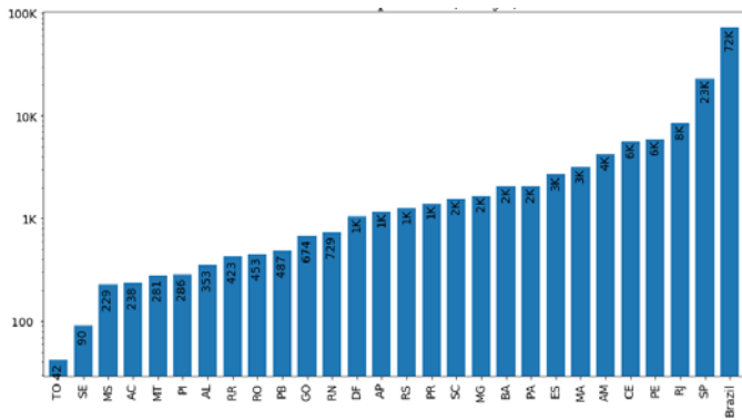
Fig 8 Short-term predict (/ days) based on GLM model
