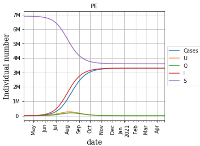
Fig 27 SUQC model of Pernambuco
