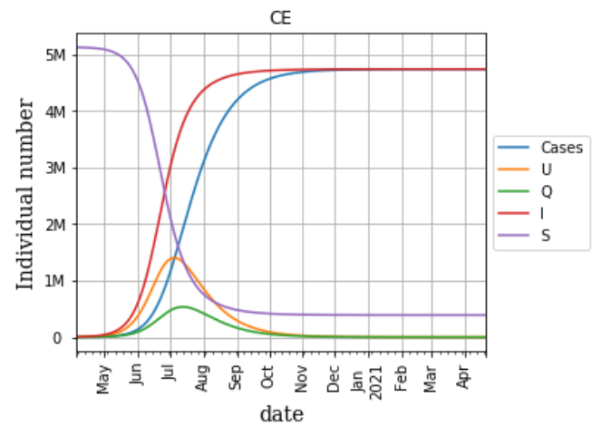
Fig 28 SUQC model of Ceara
