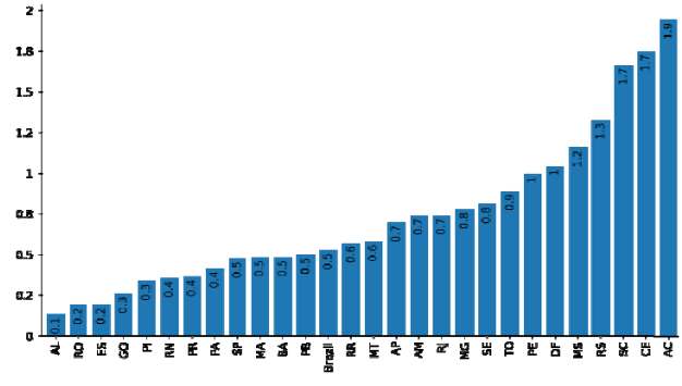
Fig 2 Growth rate based on GRM model
