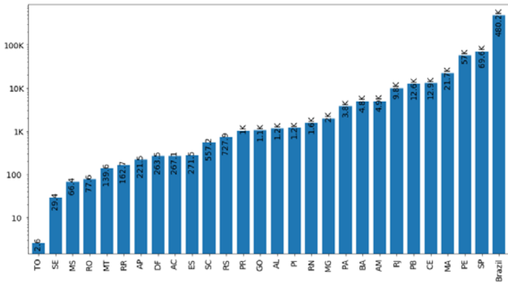
Fig 23 Total estimated deaths based on GLM model
