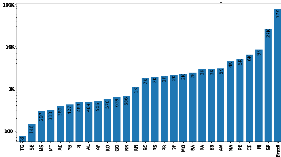
Fig 10 Short-term predict (7 days) based on SUQC model
