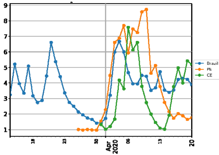
Fig 22 Growth rate (interval of 15 days) based on SUQC model
