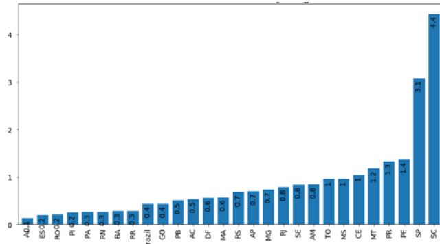
Fig 1 Growth rate based on GLM model
