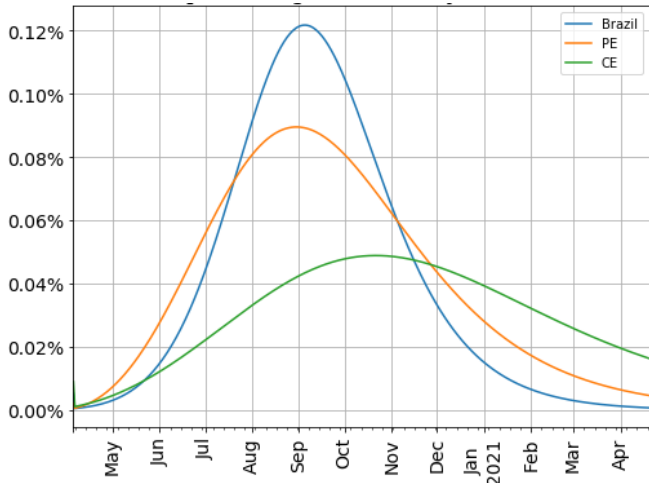
Fig 11 Percentage of daily cases based on GLM model
