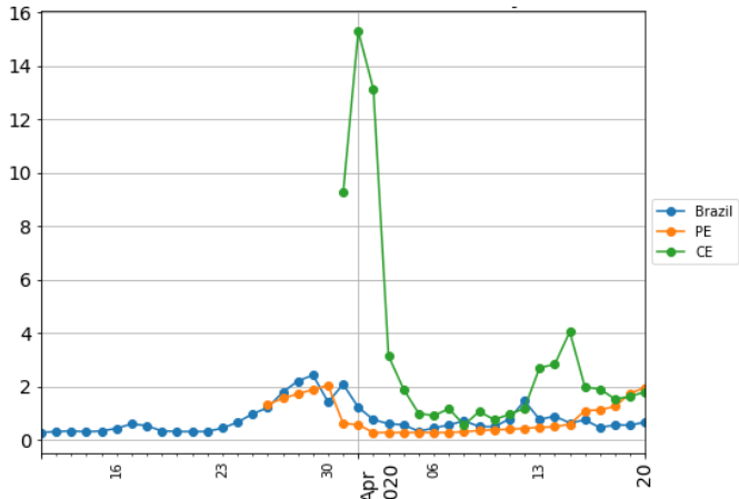
Fig 20 Growth rate (interval of 15 days) based on GLM model
