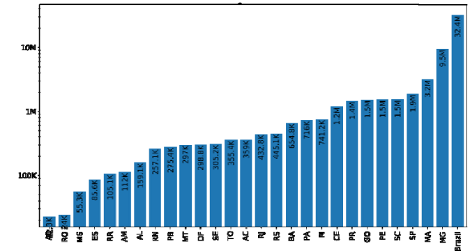
Fig 4 Final epidemic size (K) based on GRM model
