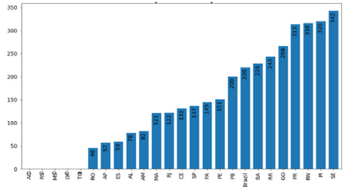
Fig 15 Number of days between start of adjustment and the peak based on GRM model
