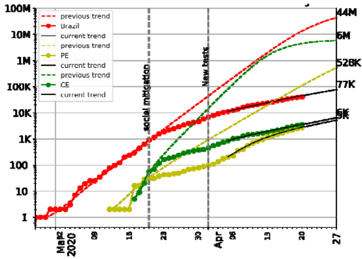
Fig 7 Forecast of the total number of cases in 7 days based SUQC model
