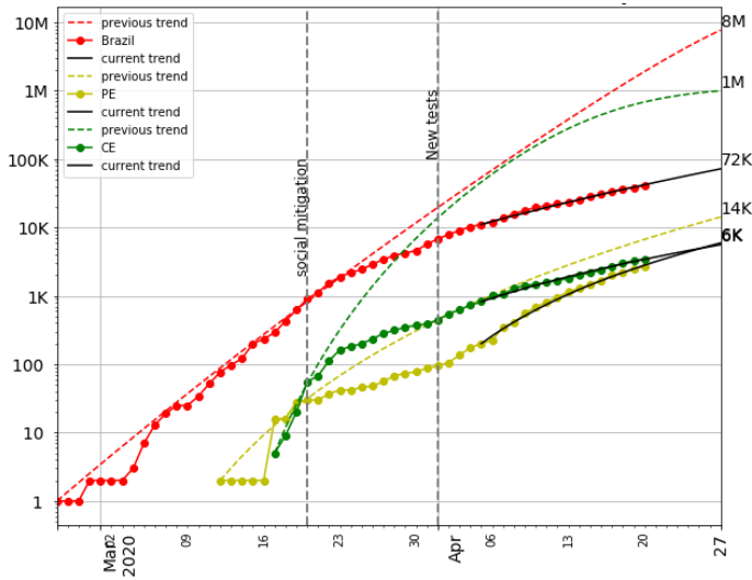
Fig 5 Forecast of the total number of cases in 7 days based on GLM model
