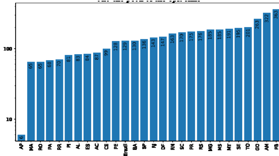
Fig 16 Number of days between start of adjustment and the peak based on SUQC model
