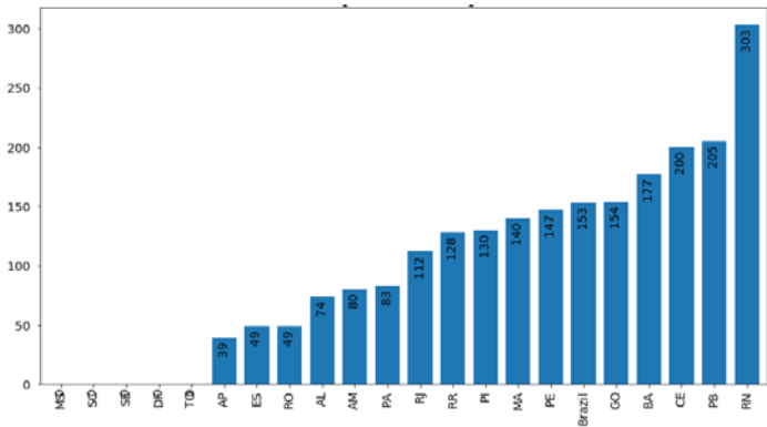
Fig 14 Number of days between start of adjustment and the peak based on GLM model
