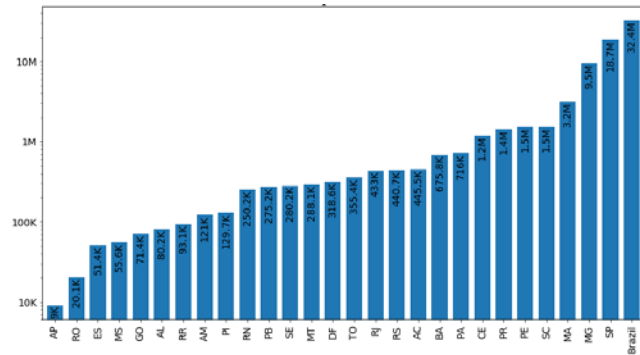
Fig 3 Final epidemic size (K) based on GLM model
