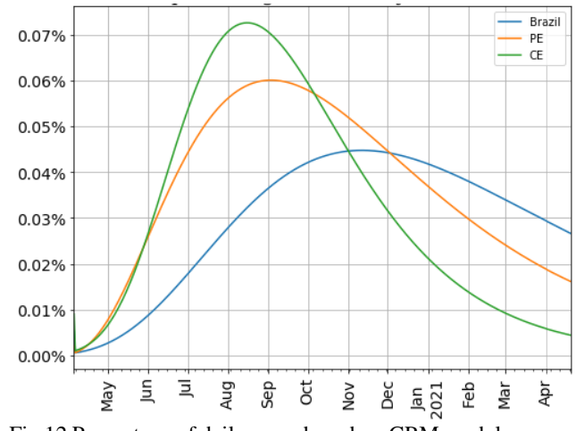
Fig 12 Percentage of daily cases based on GRM model
