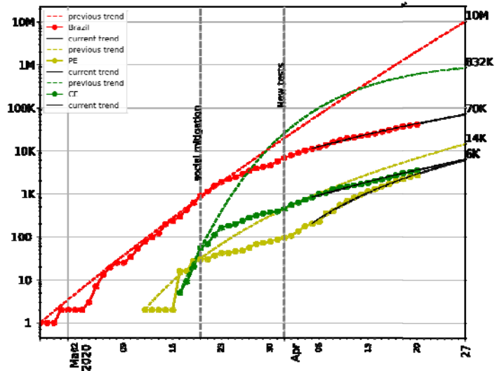
Fig 6 Forecast of the total number of cases in 7 days based GRM model
