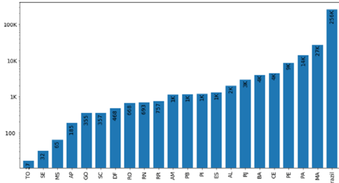
Fig 1 / Maximum number of daily cases based on GLM model
